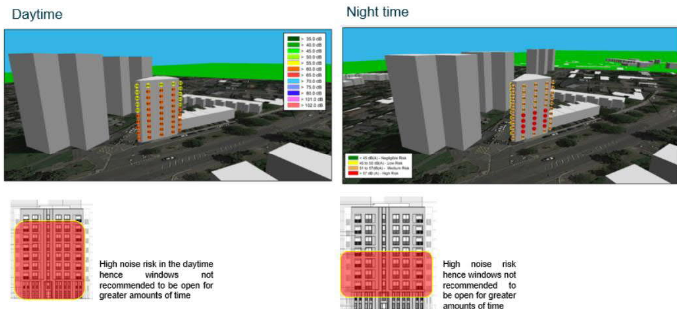
Figure 6 Acoustic Noise Risk Analysis
