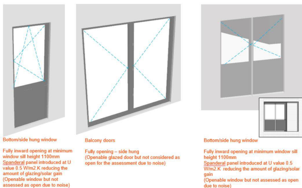
Figure 7 - Window types and opening free areas for all simulations
