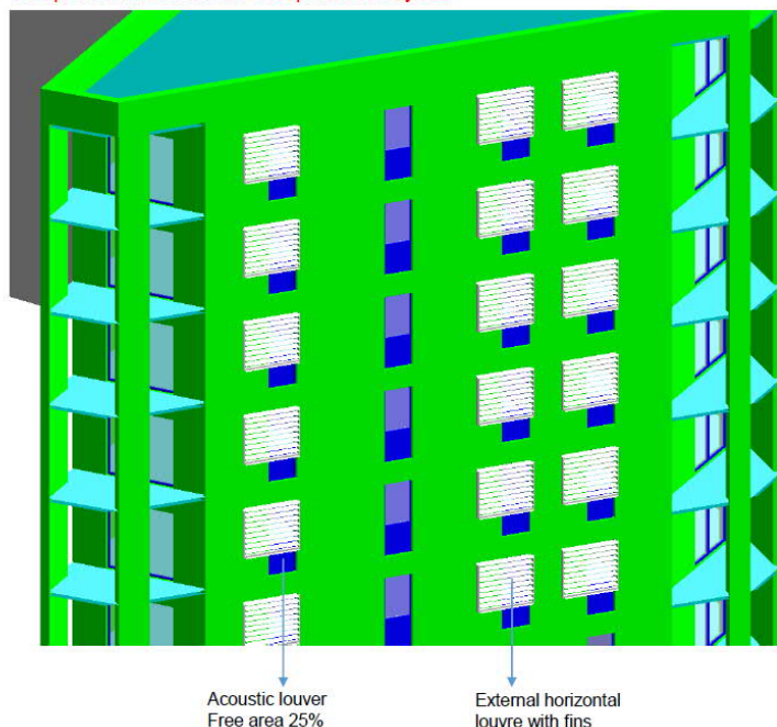
Figure 11 Louvers analysis results
