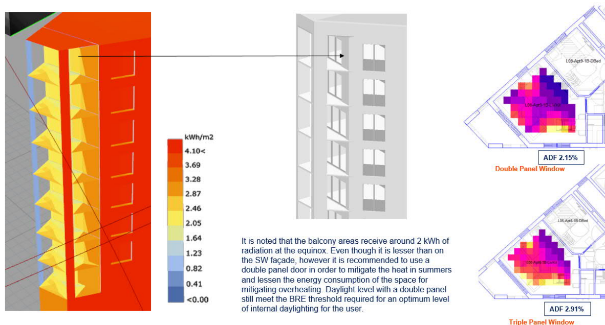
Figure 8 Optimisation study - Double Panel vs Triple Panel
