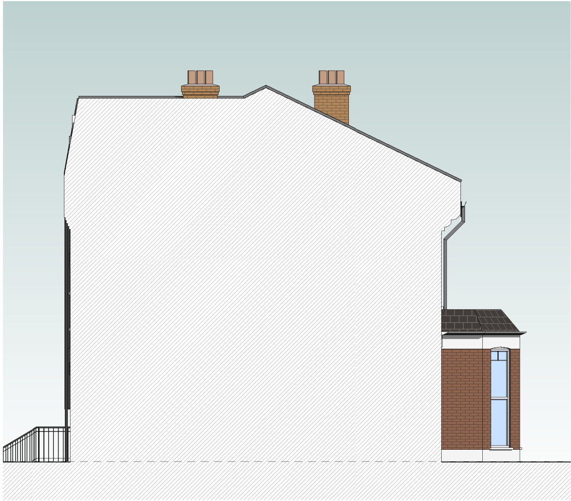
B ELEVATION B - AS EXISTING 1:100
