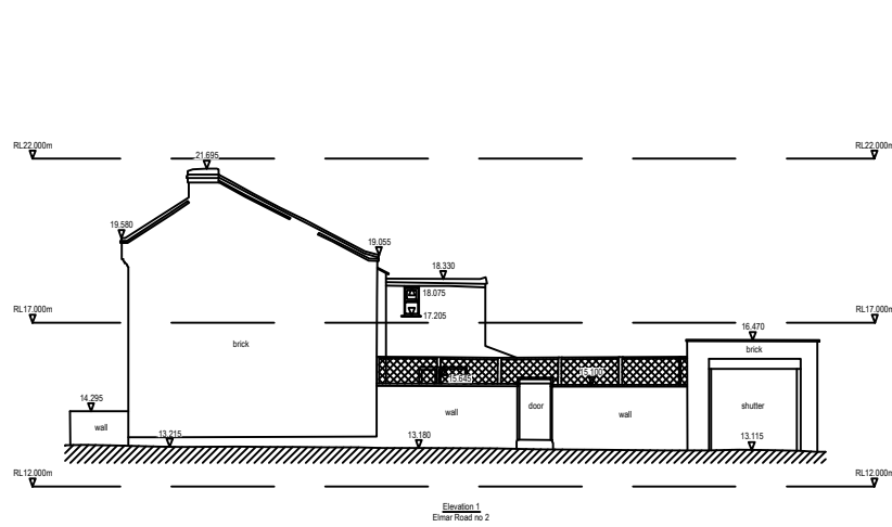
1 Existing Elevations 1:250
