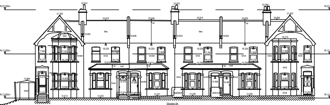
4 Existing Elevations 1:250
