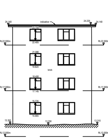
2 Existing Elevations 1:250
