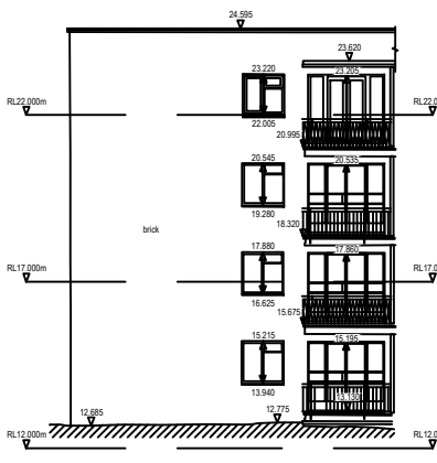
3 Existing Elevations 1:250
