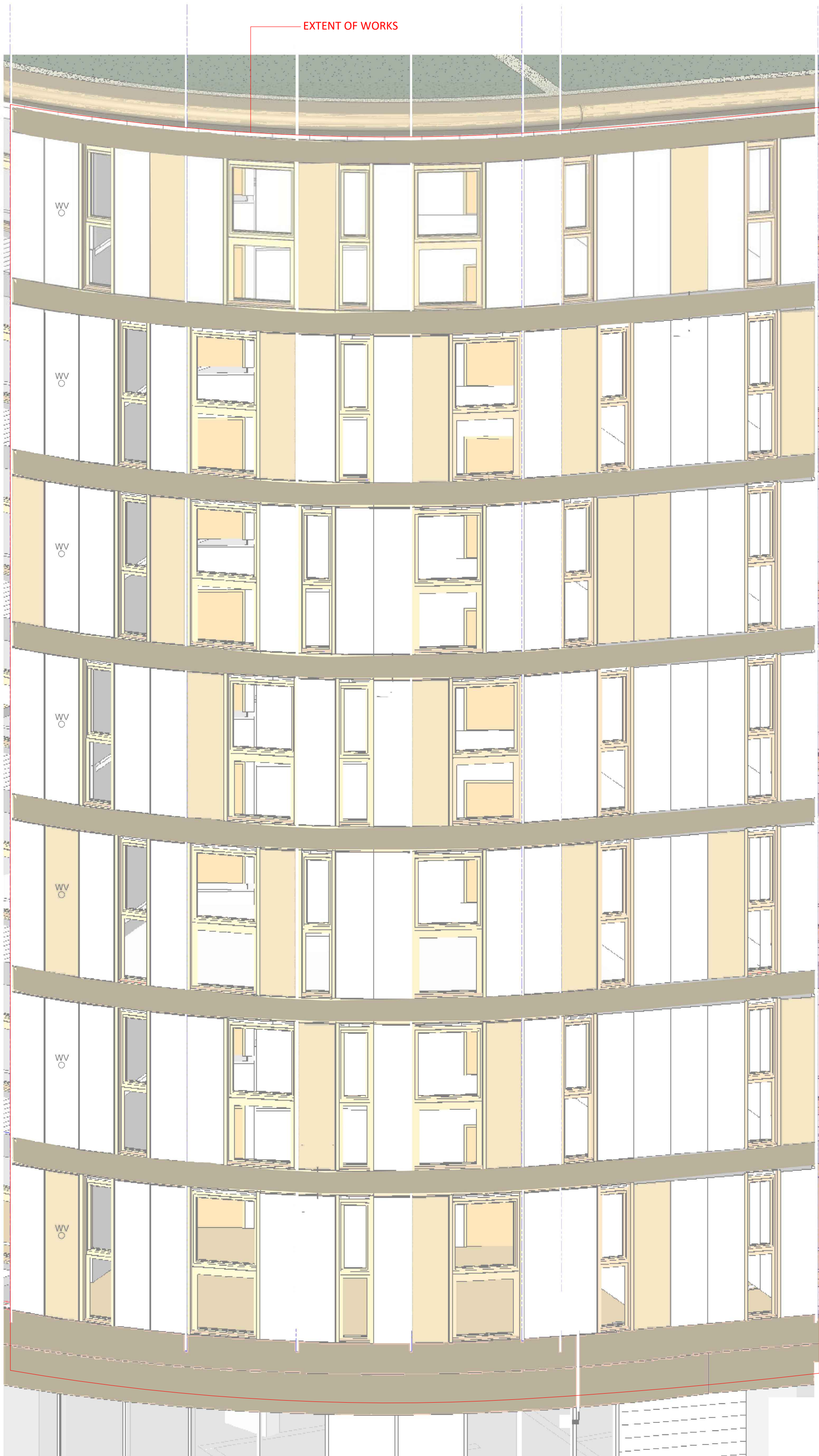
ELEVATION F - SOUTH BLOCK
