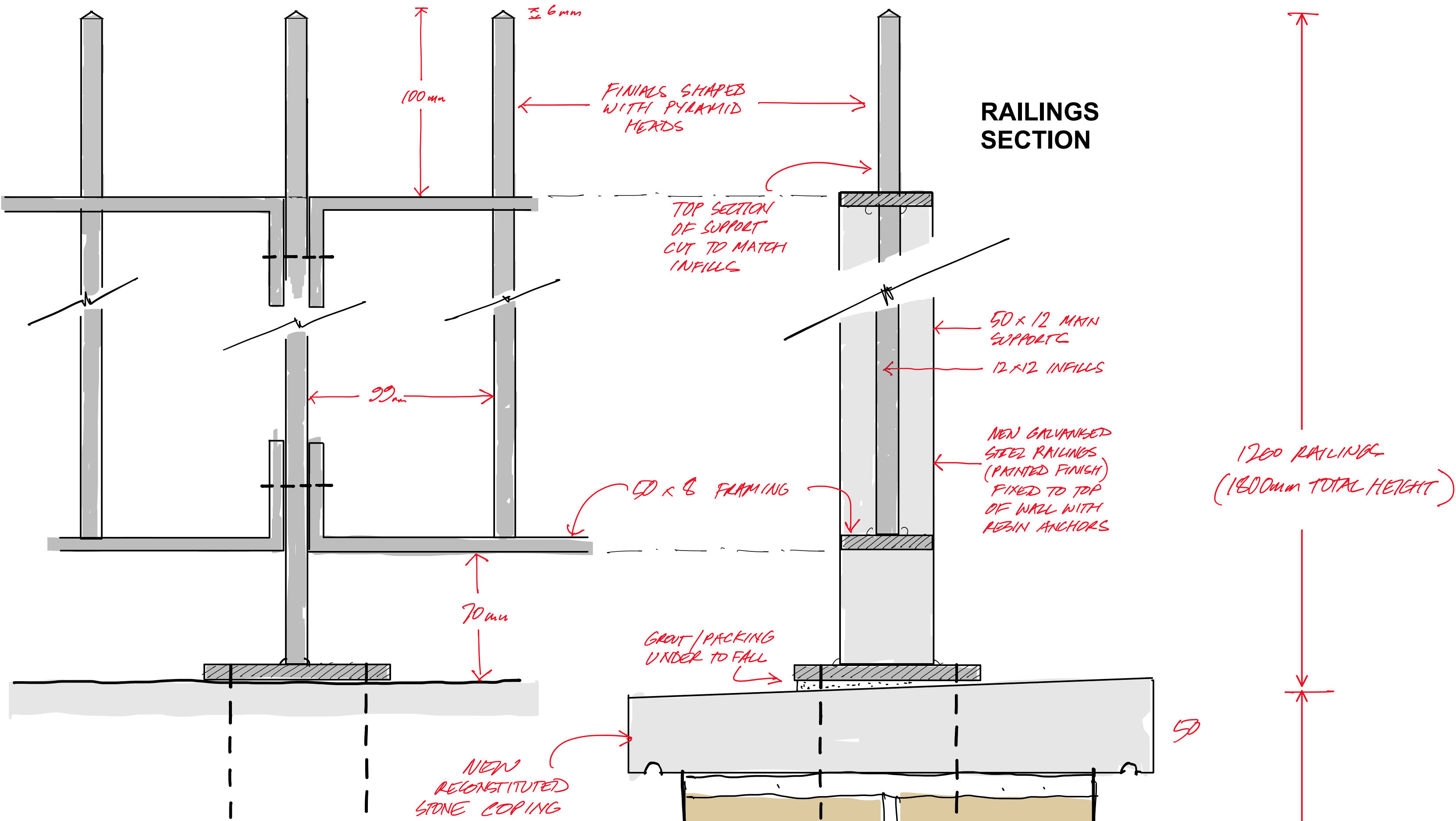
ELEVATION OF RAILINGS
