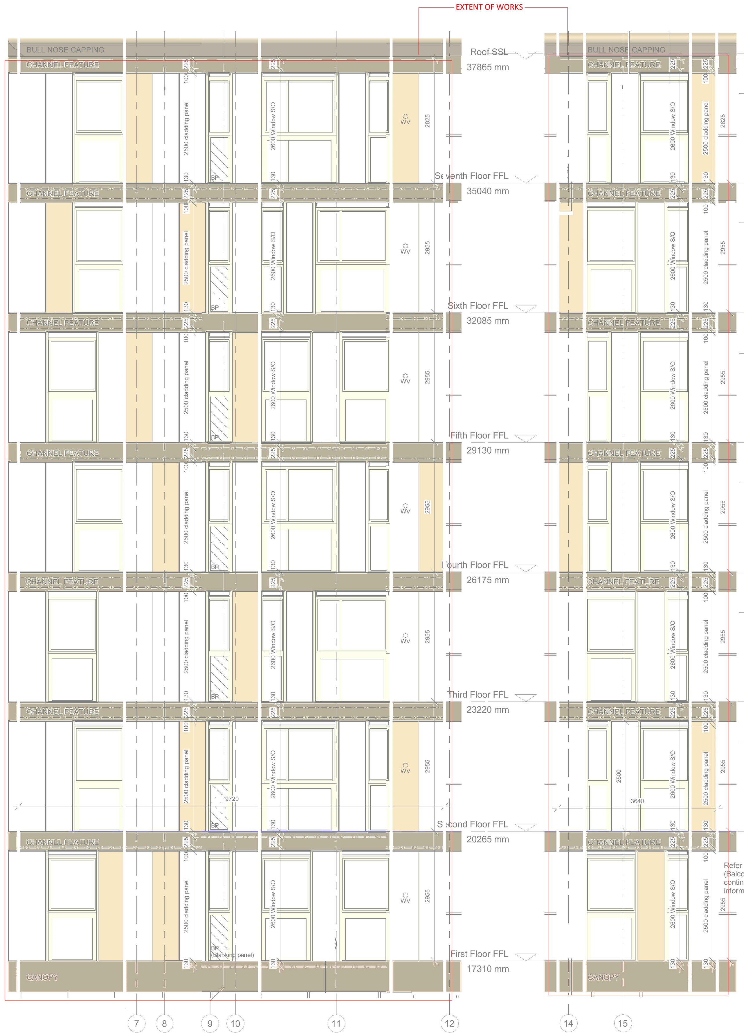
ELEVATION B - SOUTH BLOCK
