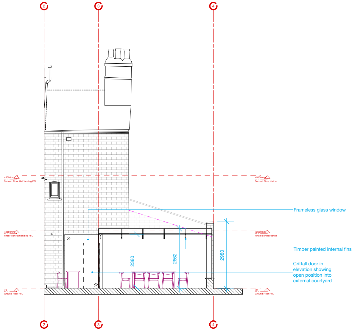
2 Proposed Side Elevation 1:100
