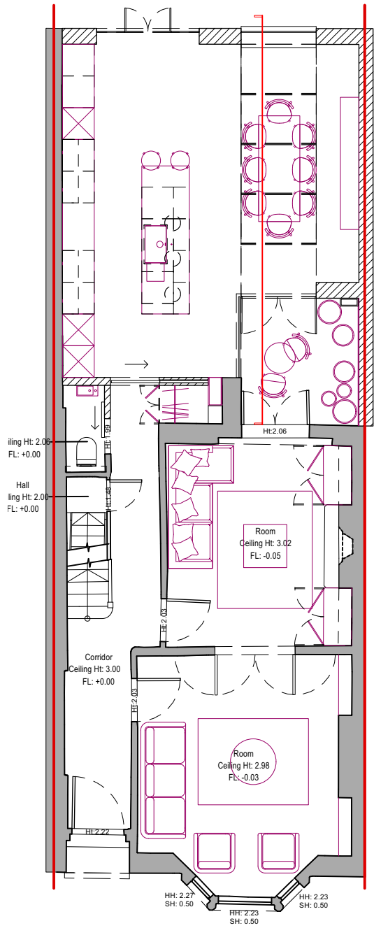
1 Reference Plan 1:100
