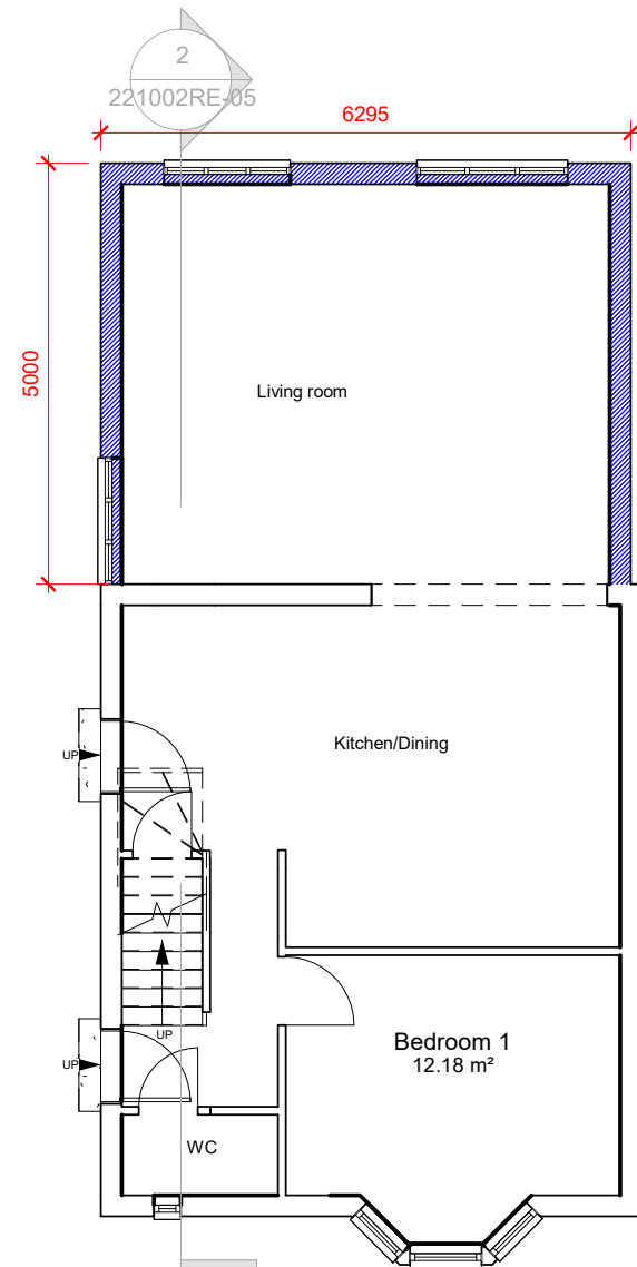
01. GF Proposed 1 : 100
