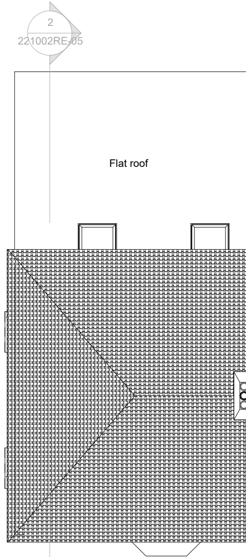
04. RF Proposed 1 : 100
