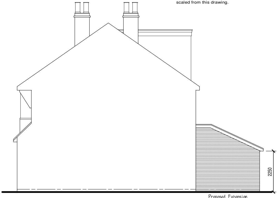
SIDE ELEVATION
