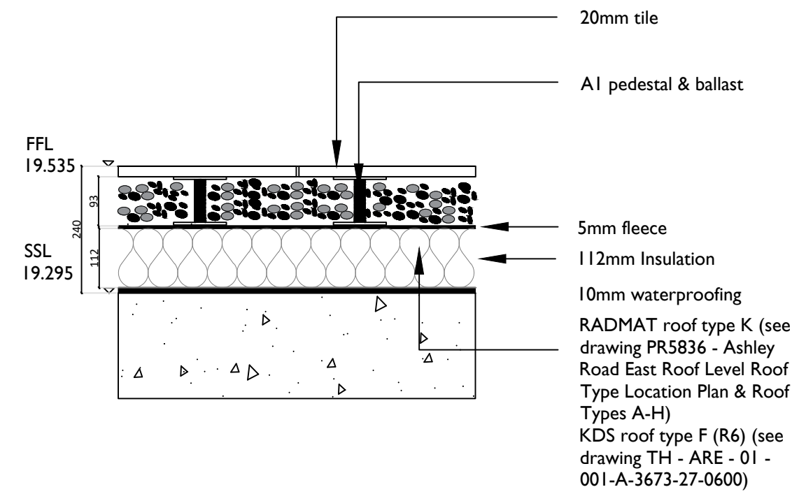
Level 2 Roof type K Tiles on pedestals Deepest profile
