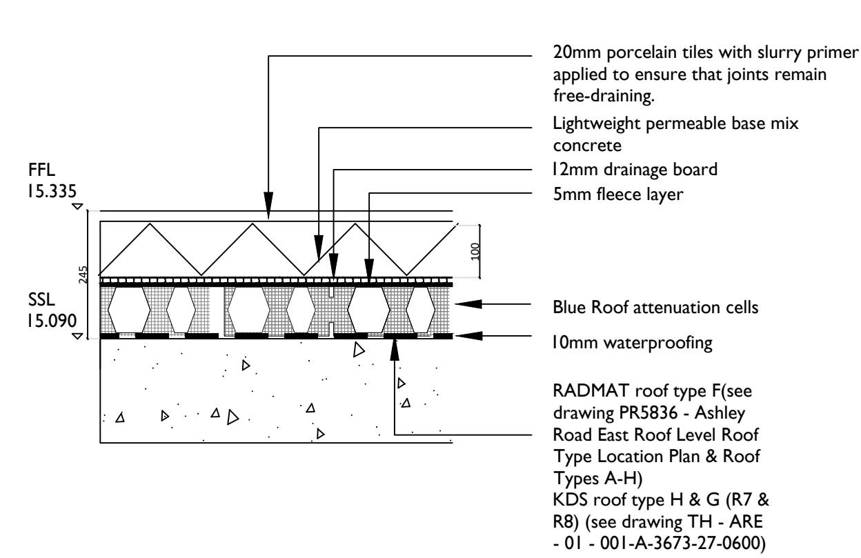
Level 1 Roof type F Shallowest build-up
