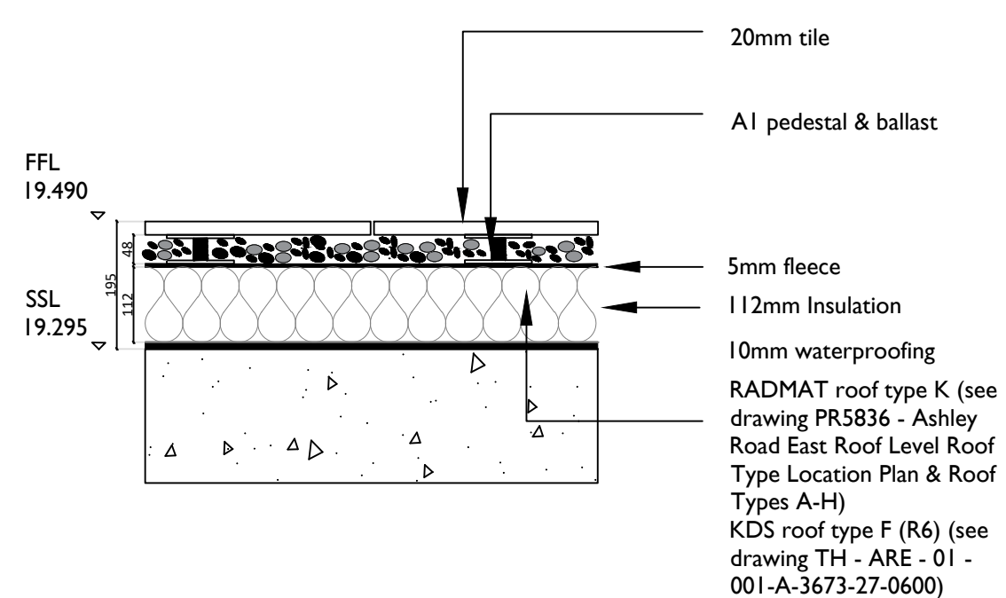
Level 2 Roof type K Tiles on pedestals Shallowest profile
