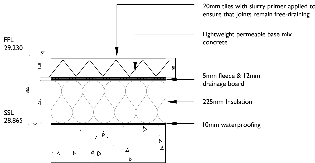
Level 5 Roof type C Deepest build-up
