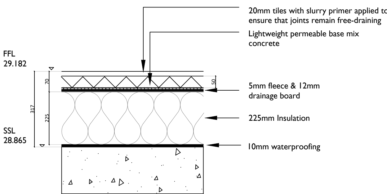
Level 5 Roof type C Shallowest build-up
