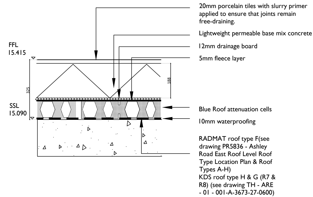
Level 1 Roof type F Deepest build-up
