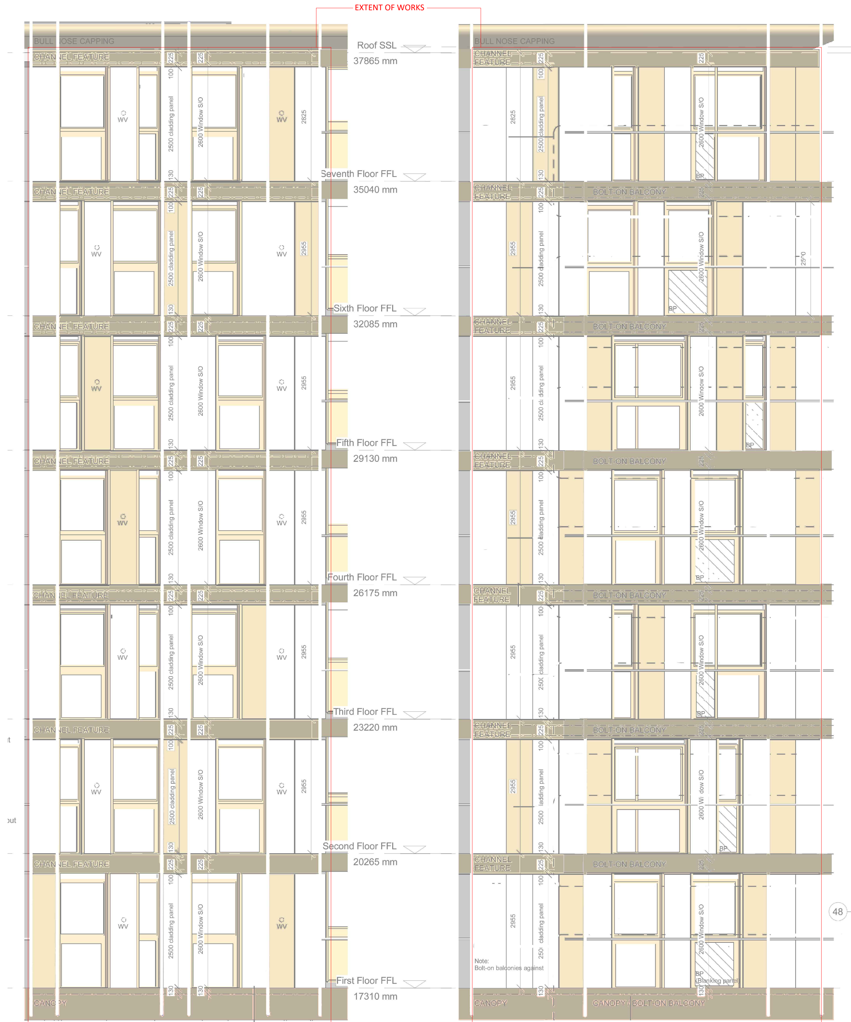
ELEVATION G - SOUTH BLOCK
