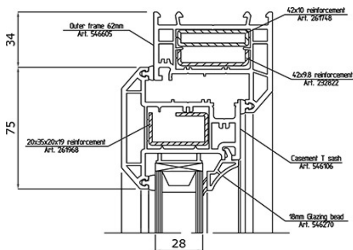
L-L Section Detail
