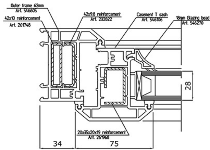
P-P Section Detail
