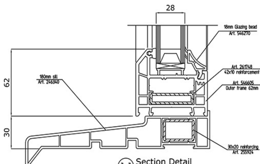
R-R Section Detail
