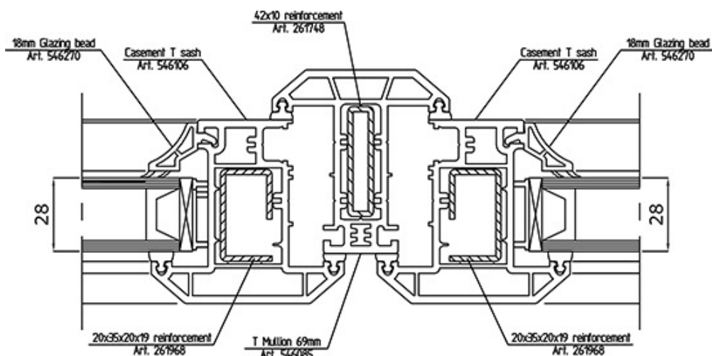
R-R Section Detail
