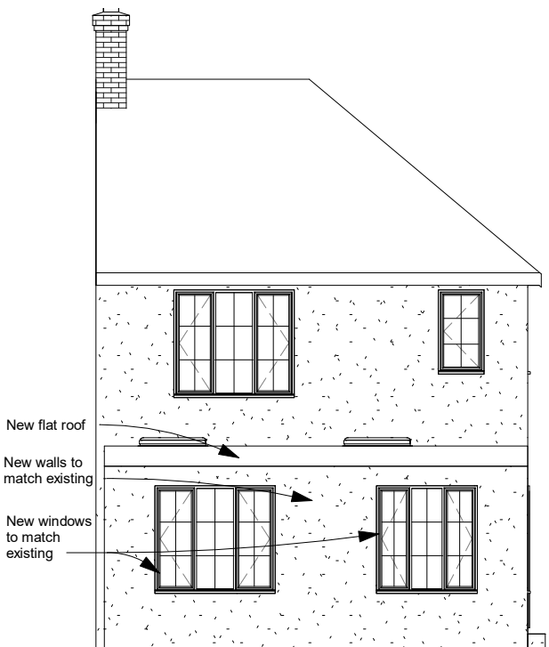
02. Rear Elevation Proposed 1 : 100
