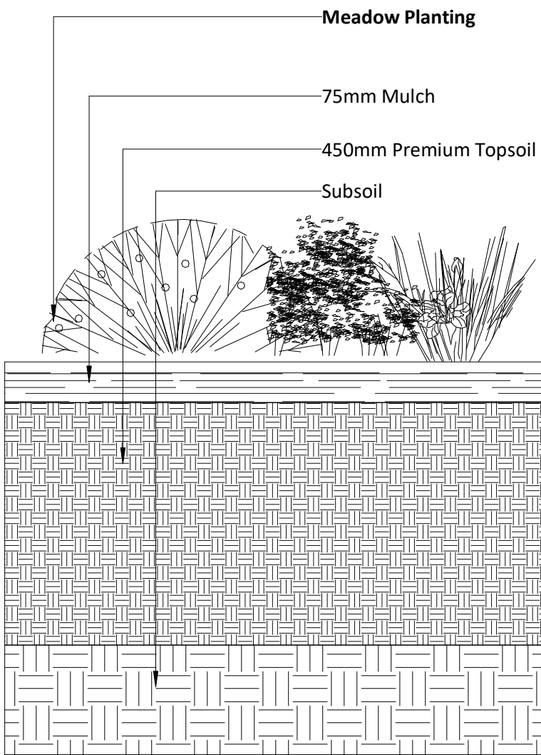
Detail 10 - Proposed Meadow Planting 1 : 10
