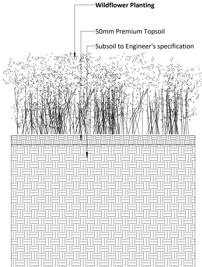
Detail 09 - Typical Wildflower Planting Detail 1 : 10
