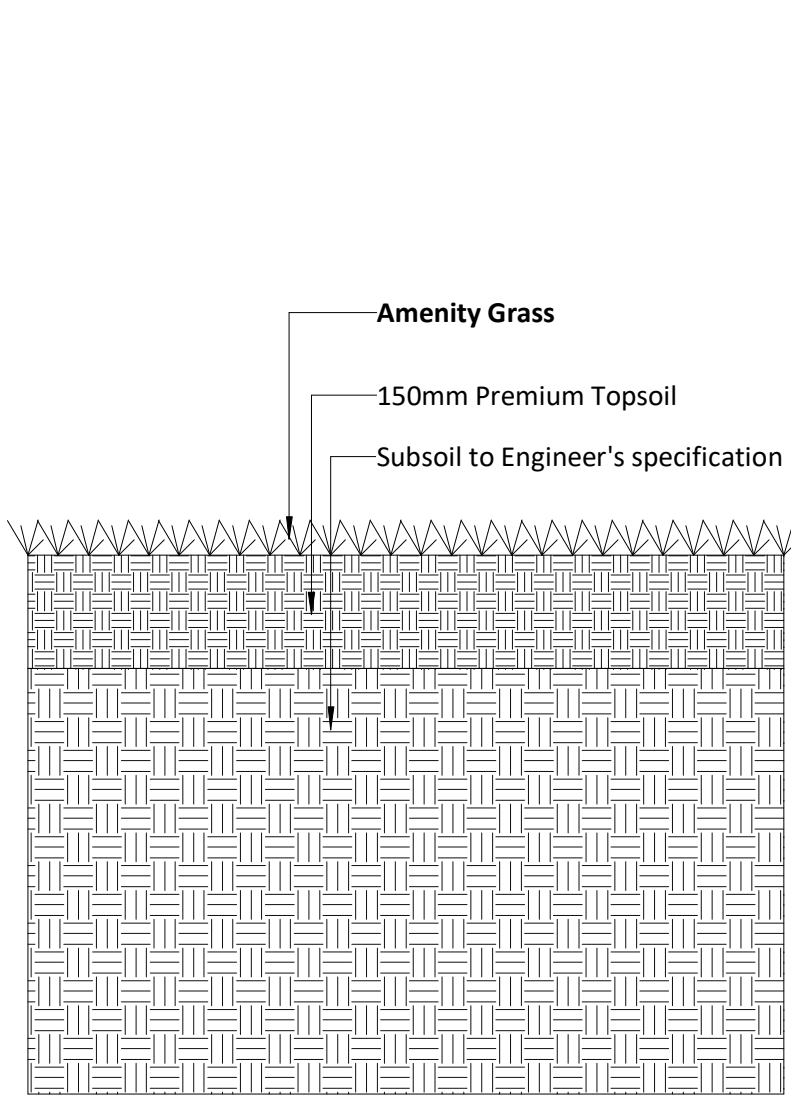
Detail 08 - Proposed Amenity Grass 1 : 10
