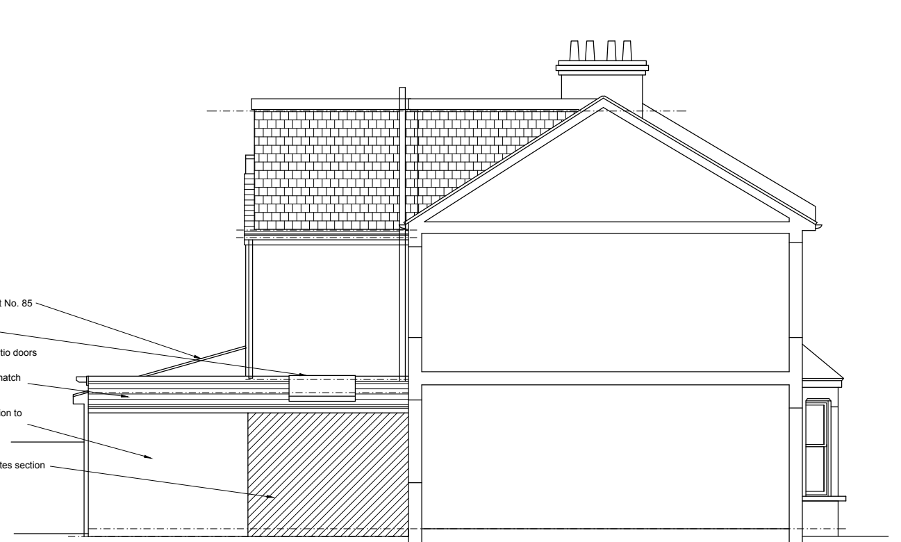
PROPOSED SIDE ELEVATION / SECTION
