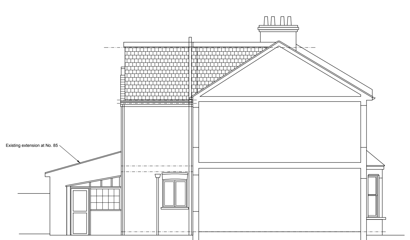
EXISTING SIDE ELEVATION / SECTION
