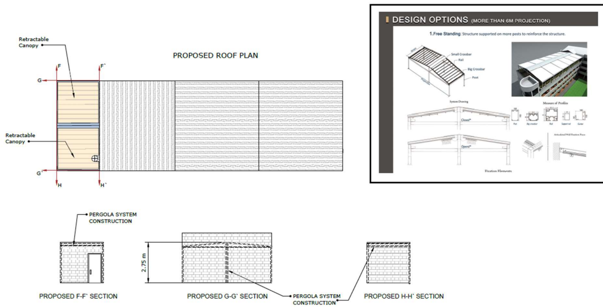
Figure 2. Proposed Pergola System
