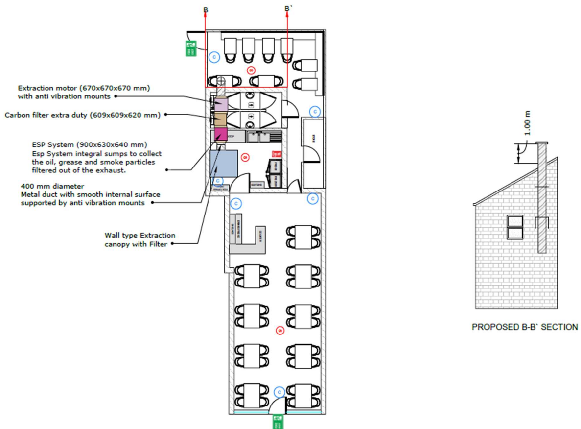
Figure 1. Proposed Flue System
