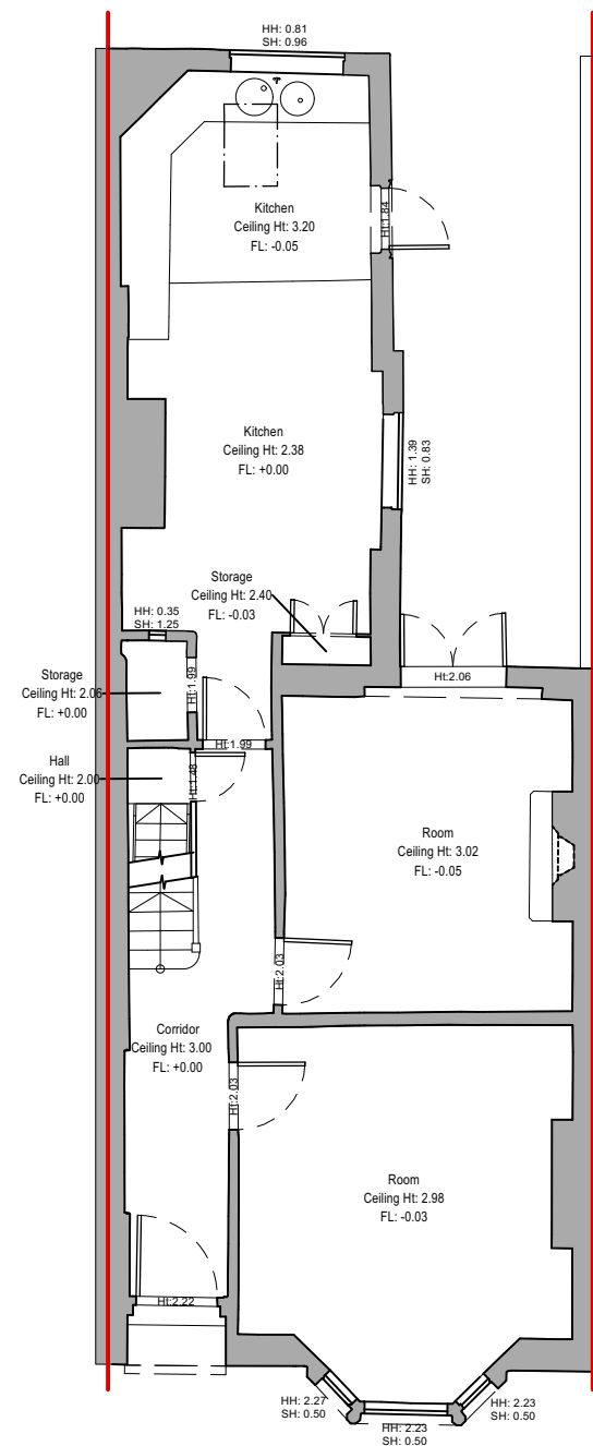
1 Reference Plan 1:100
