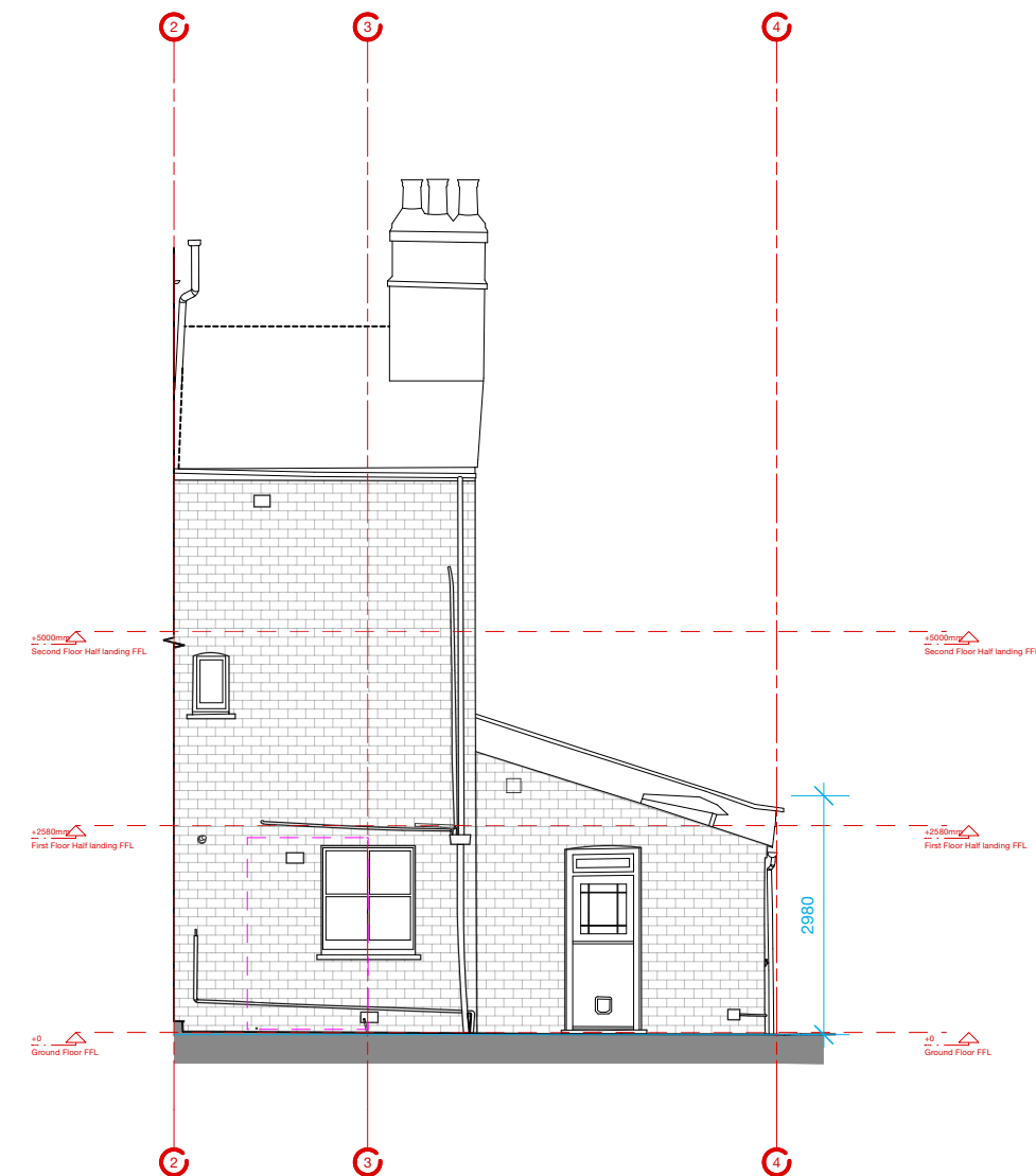
2 Existing Side Elevation 1:100
