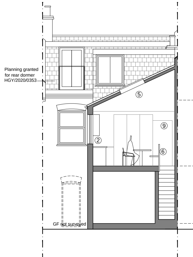
SECTION BB
