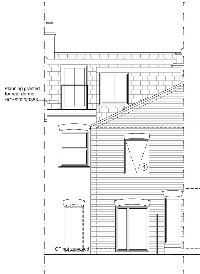
REAR ELAVATION
