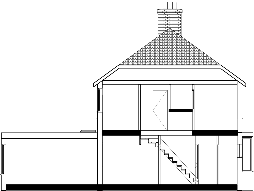
Section Proposed 1 : 100
