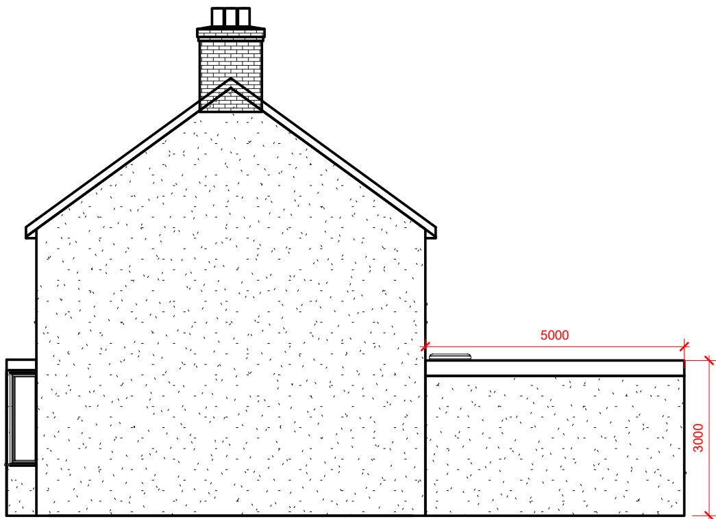
03. Right Elevation Proposed 1 : 100
