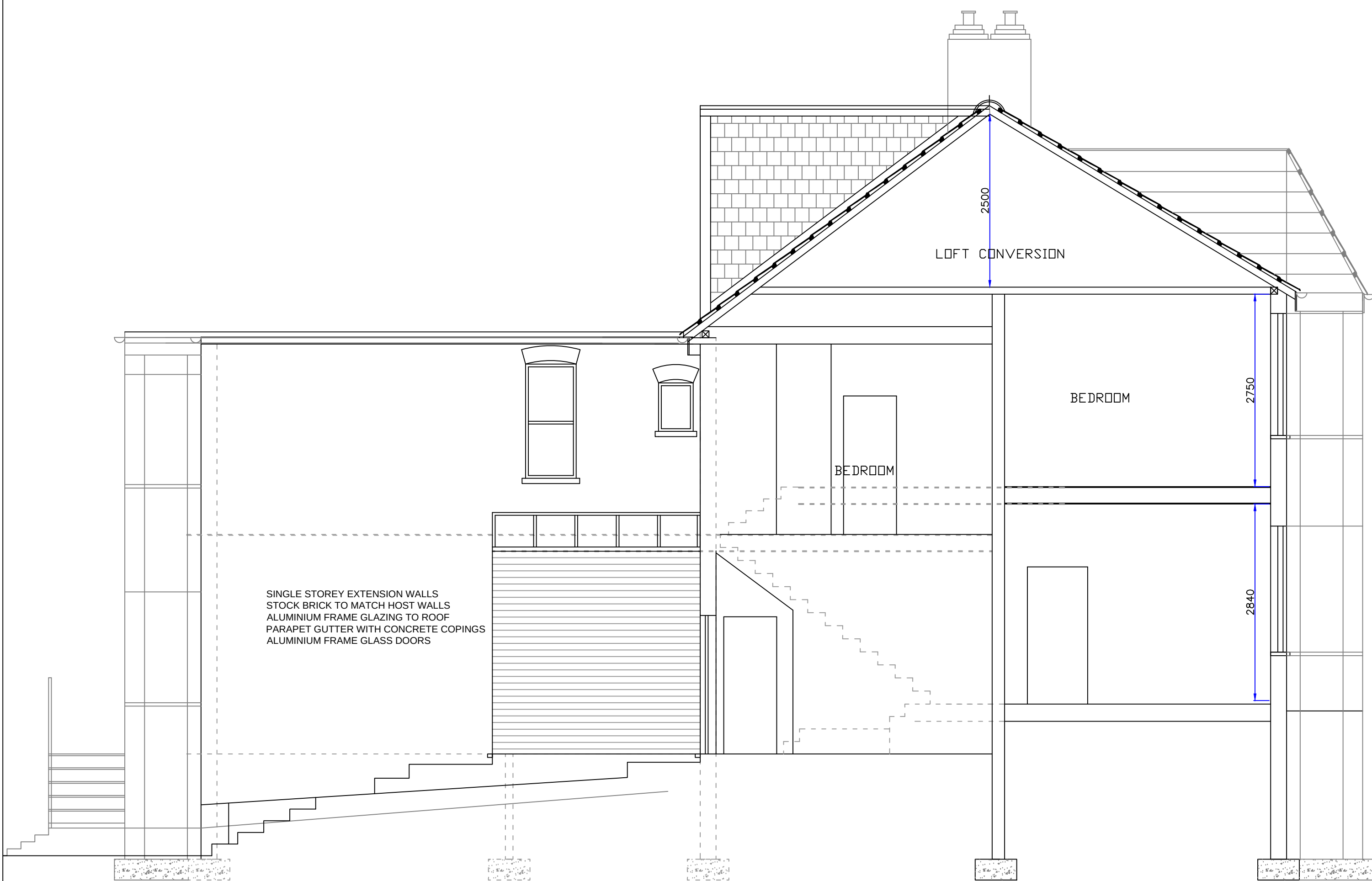
PROPOSED SIDE EXTENSION 1:50
