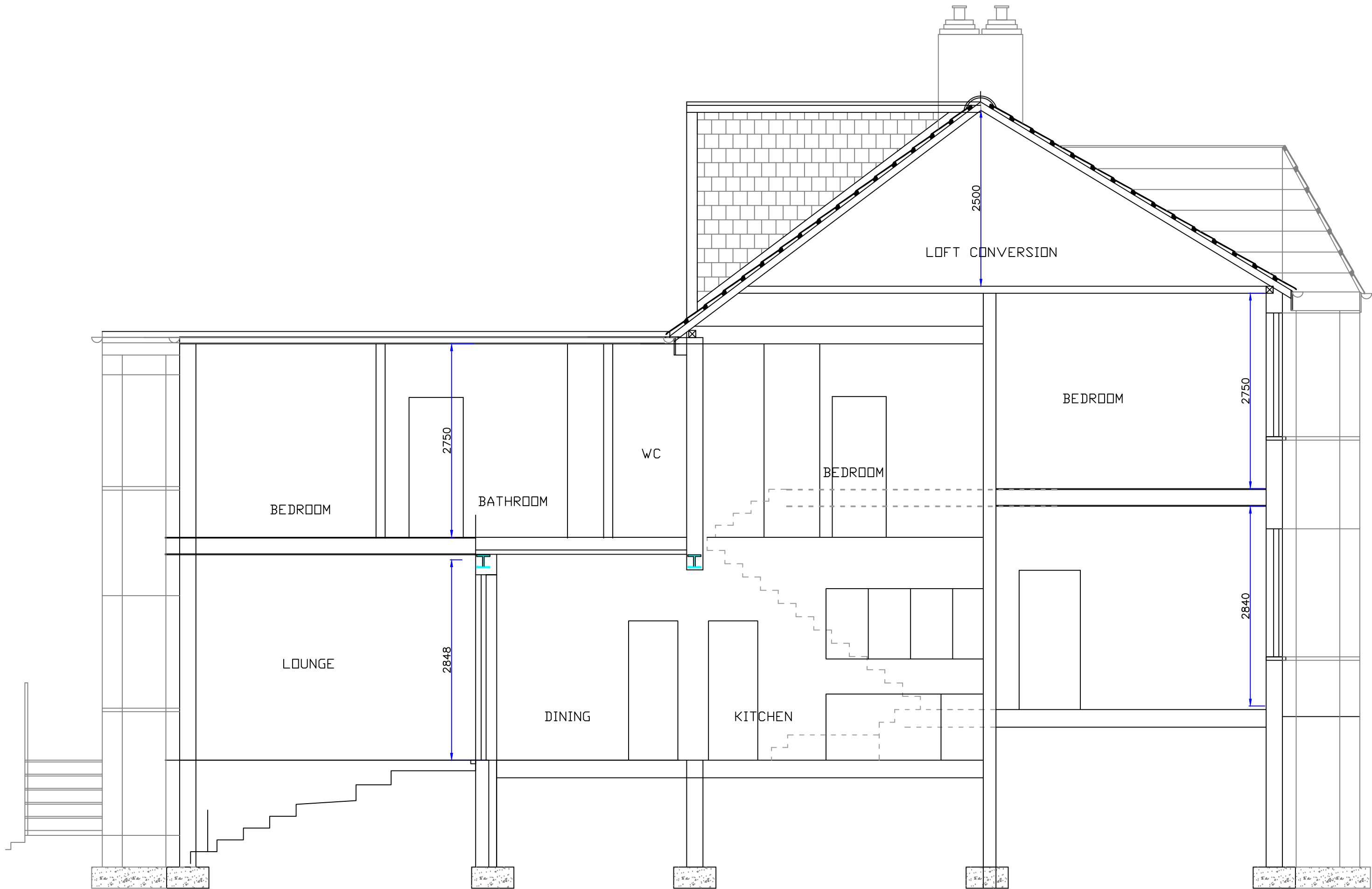
PROPOSED LONG SECTION 1:50
