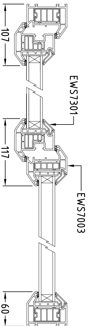
Section X-X Scale 1:4
