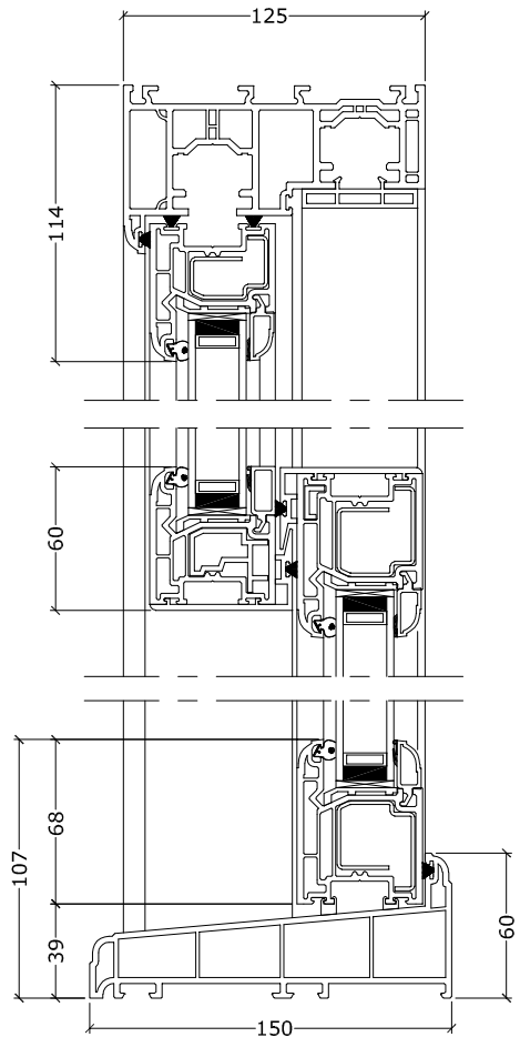
C-C Section Detail
