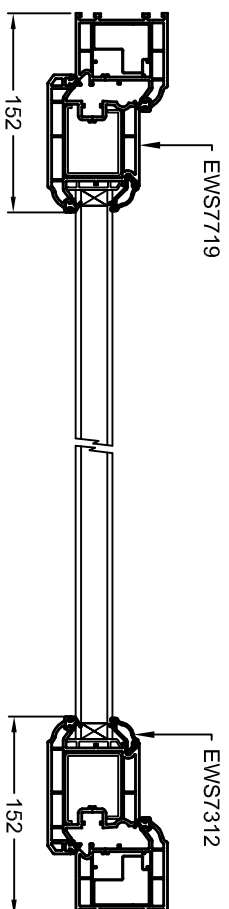
Section X-X Scale 1:4
