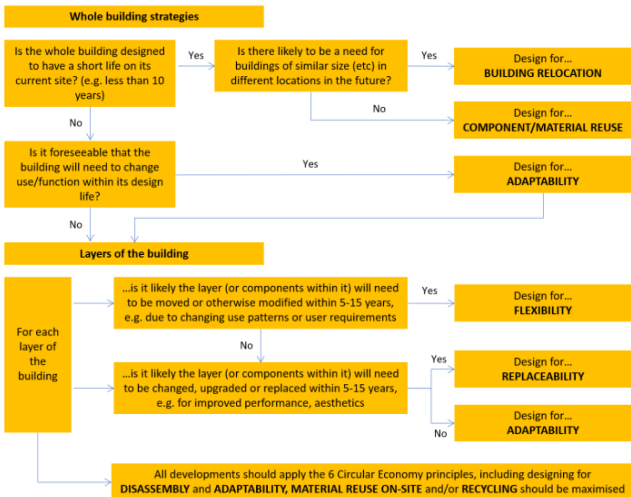
Figure 5: Decision Tree for Design Approaches for New Buildings, Infrastructure and Layers Over Lifetime of Development
