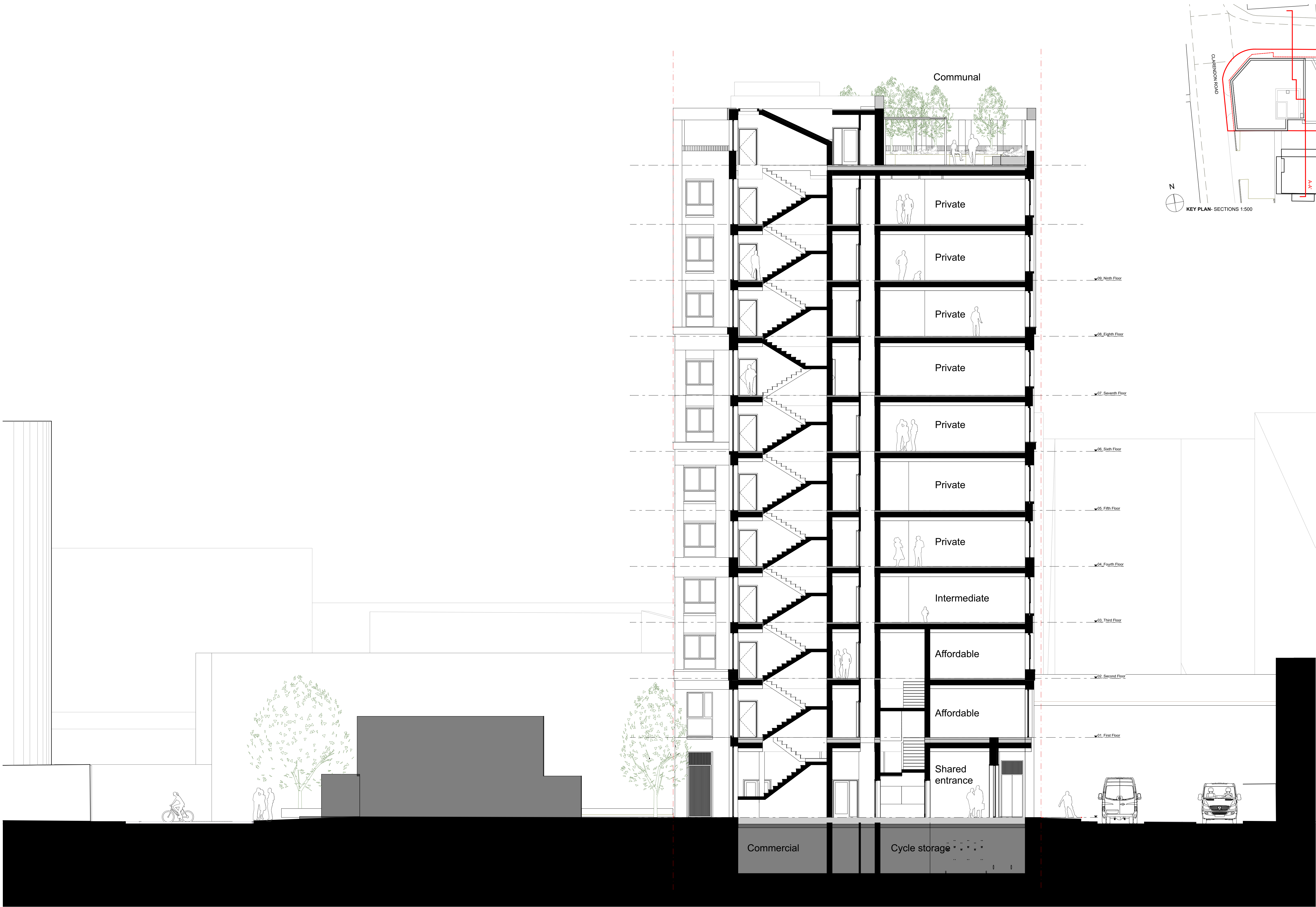
0 6 12 18m A-A' EAST - WEST SECTION
