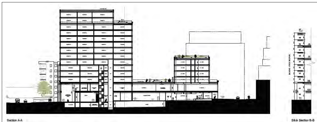
Proposed section of the new building including single level basement (extract from section drawing ref 3510-AL(20)400, dated May 2020, created by Stock Wool architects and provided by Graphic Structures).
