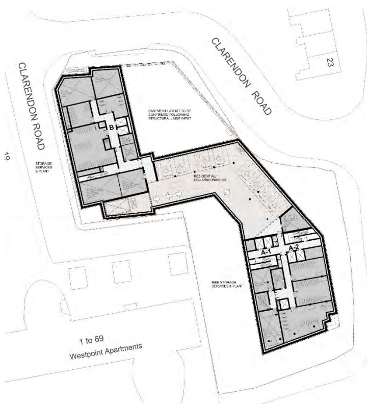
BASEMENT PLAN PREVIOUS SCHEME (DECEMBER 2020)
