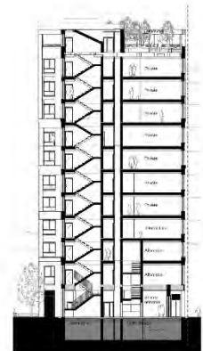
N-S SECTION NEW SCHEME
