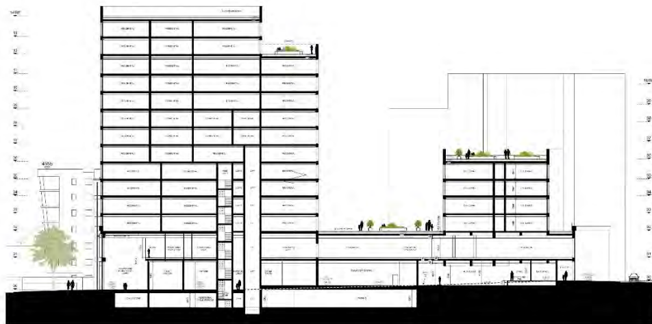
N-S SECTION PREVIOUS SCHEME (DECEMBER 2020)
