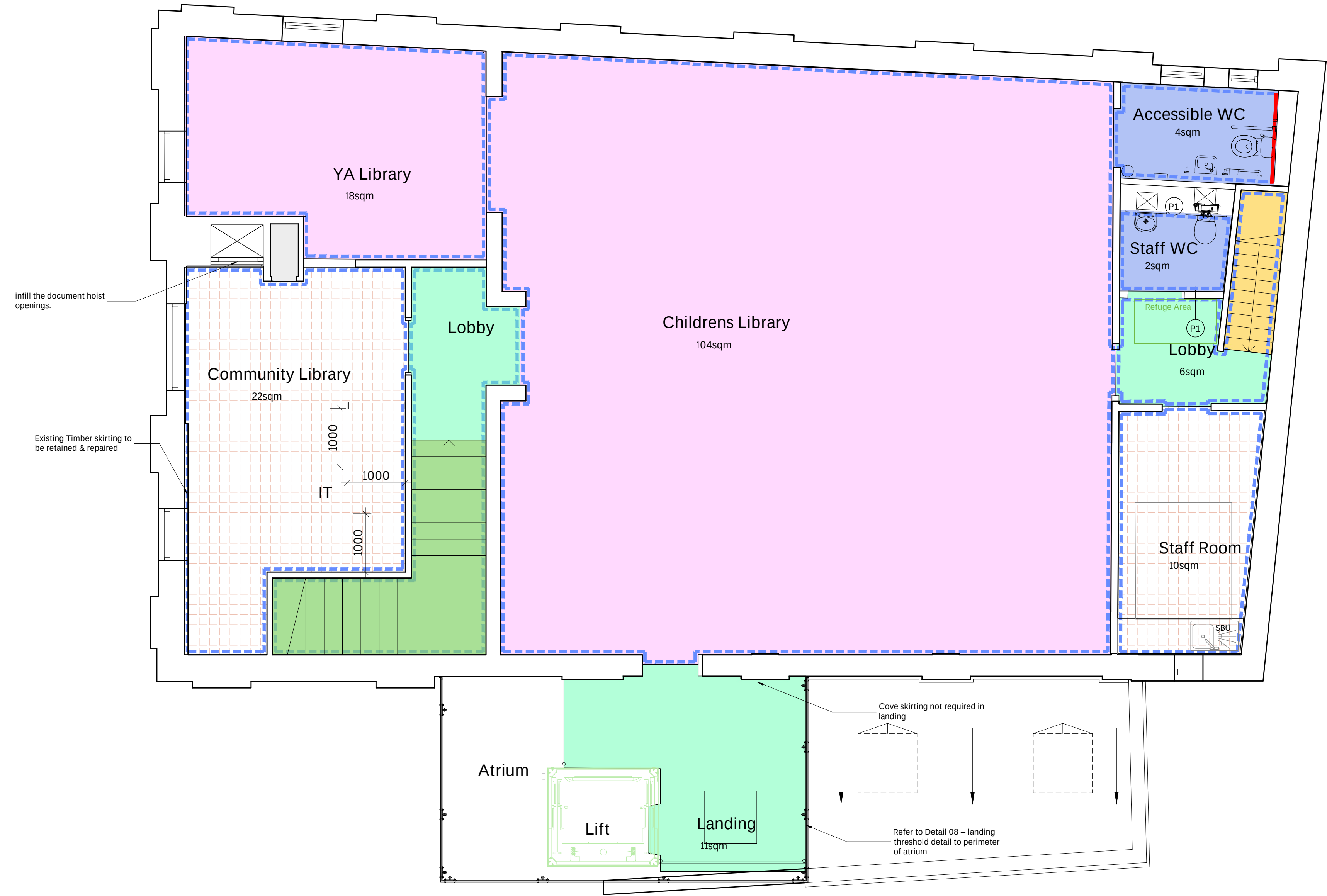
First Floor Floor and Wall Finishes
