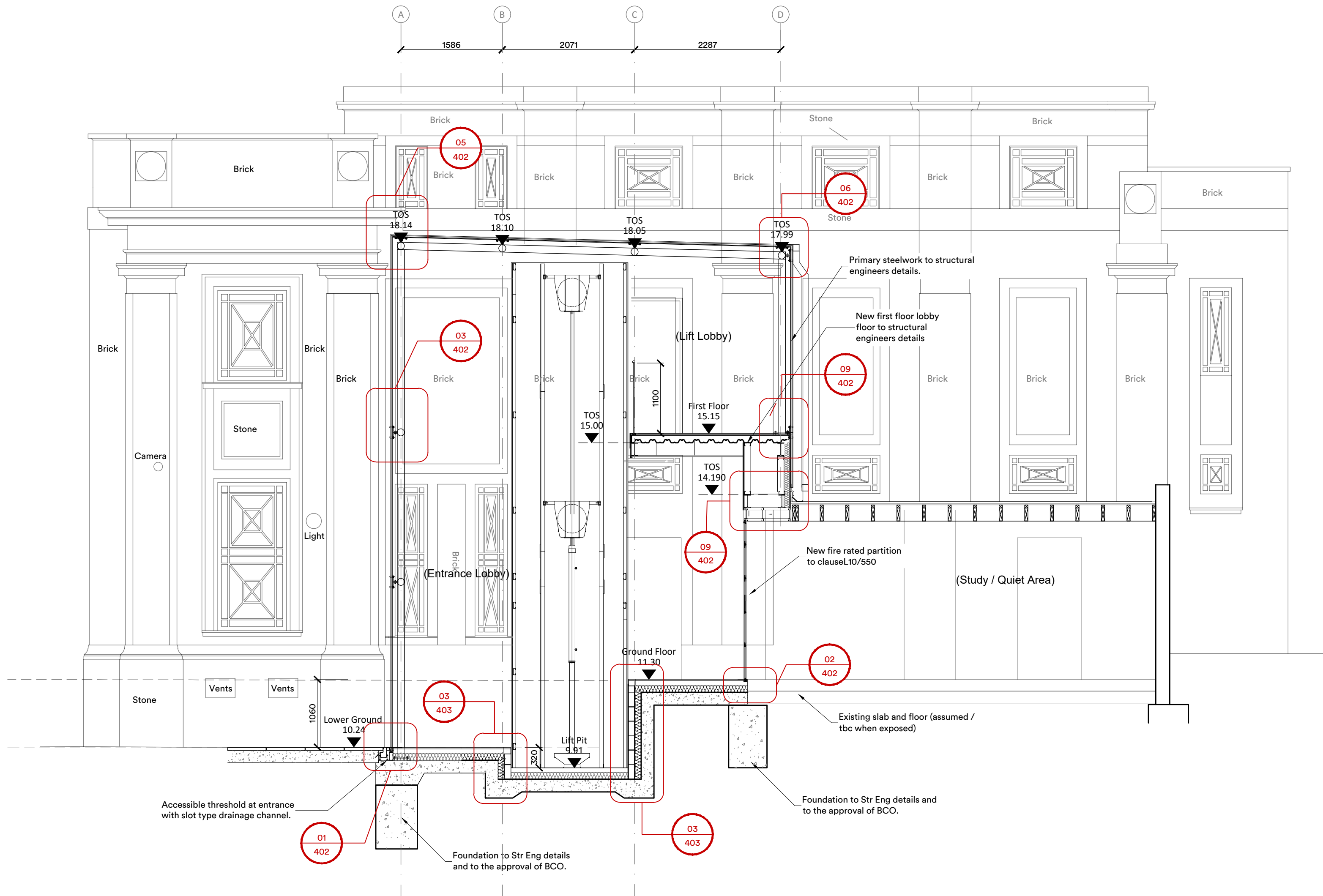
Section CC As Proposed
