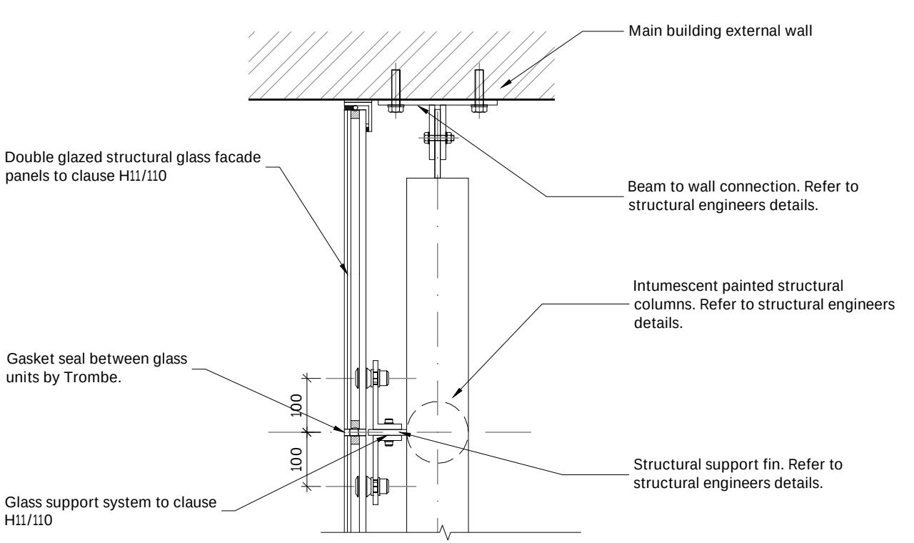
Detail 11 Typical vertical glass junction 1:10
