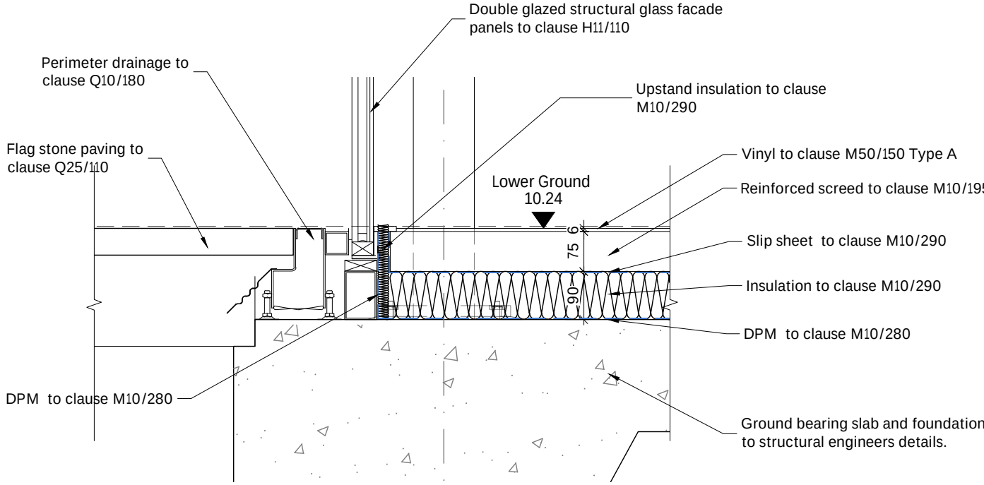
Detail 01 Typical Perimeter Detail 1:10
