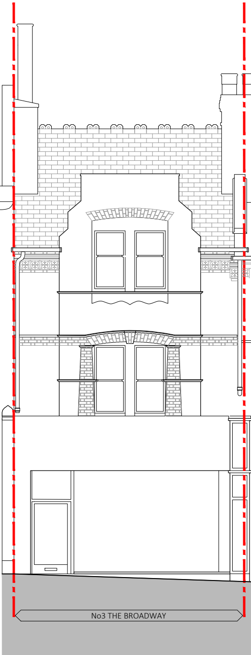
1 Existing Front Elevation 1:100 @ A3
