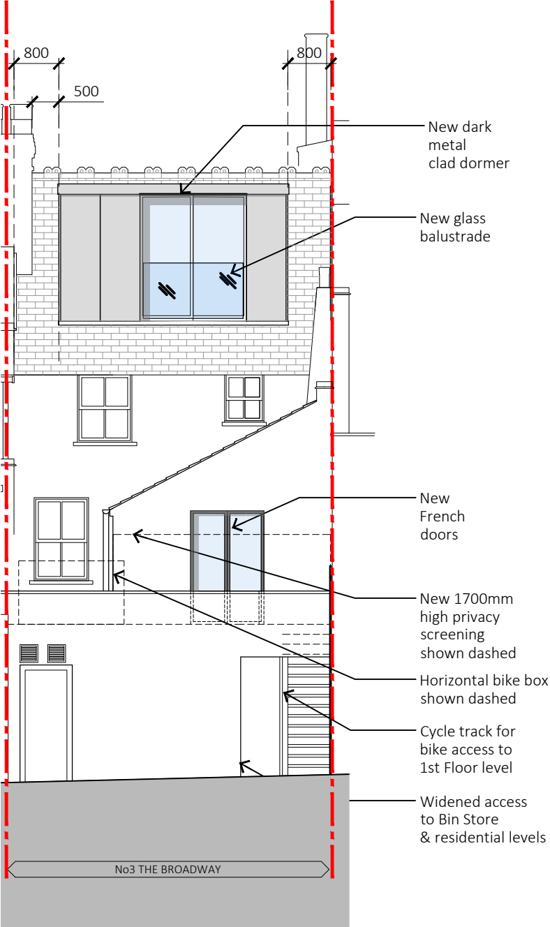
2 Proposed Rear Elevation 1:100 @ A3
