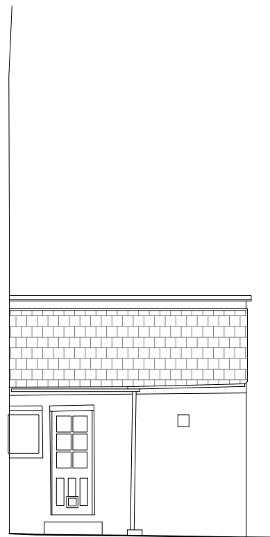
SIDE ELEVATION
