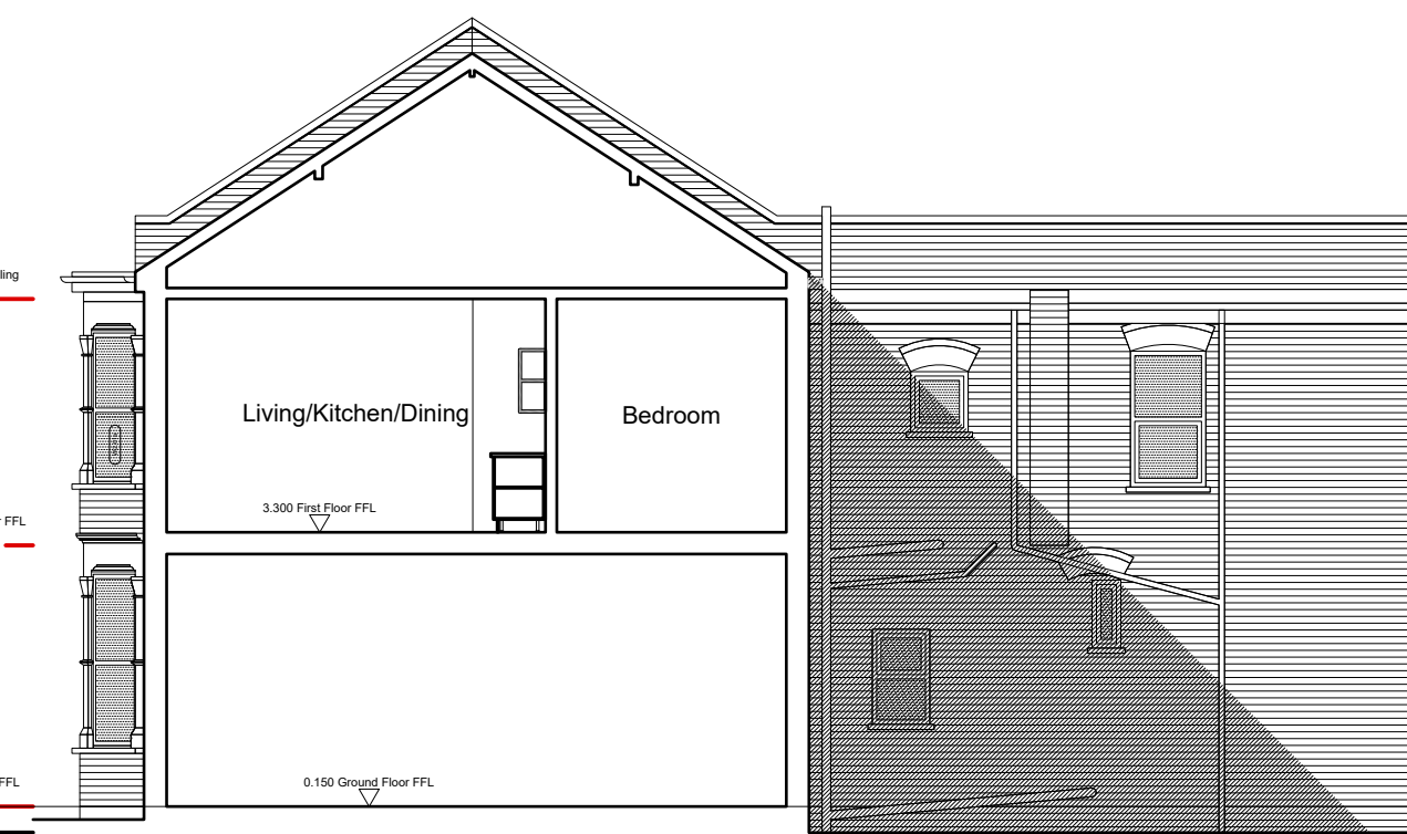
Side Elevation
