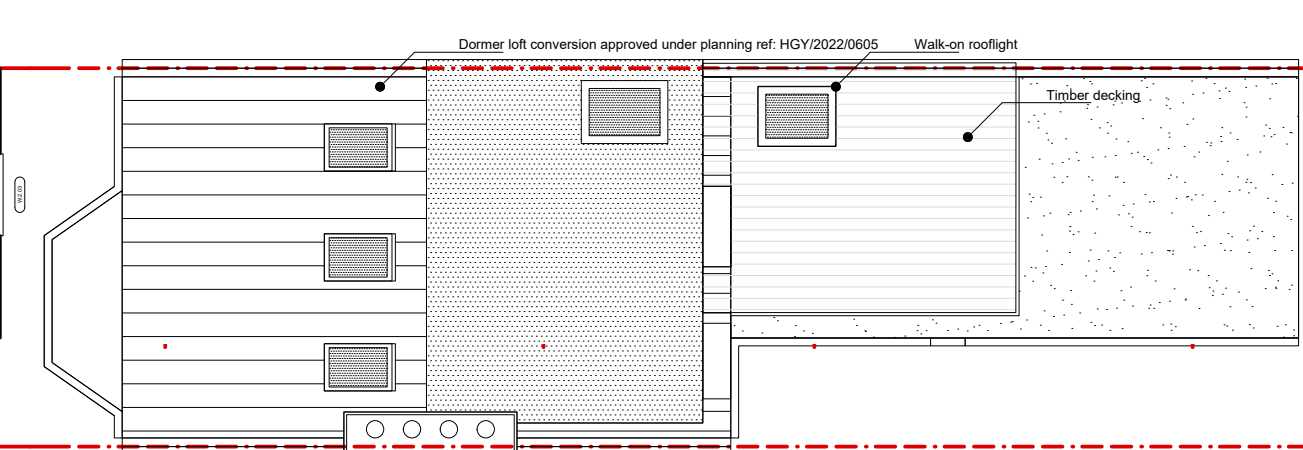
Roof Plan
