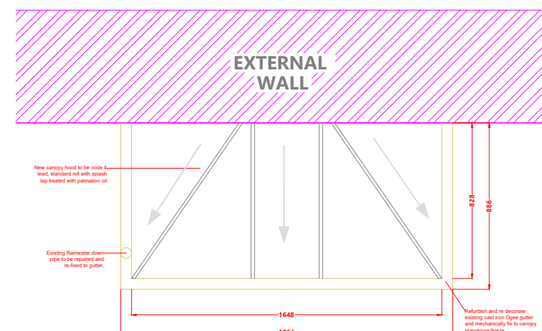
PORCH CANOPY HOOD - PROPOSED
