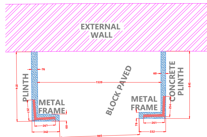
PORCH CANOPY FOOTINGS - EXISTING
