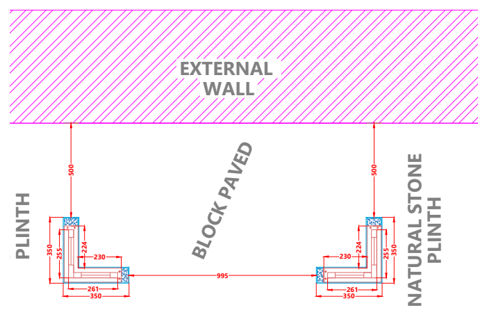
PORCH CANOPY FOOTINGS - PROPOSED
