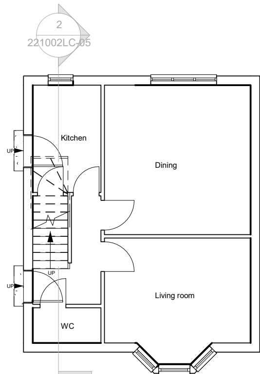
01. GF Proposed 1 : 100
