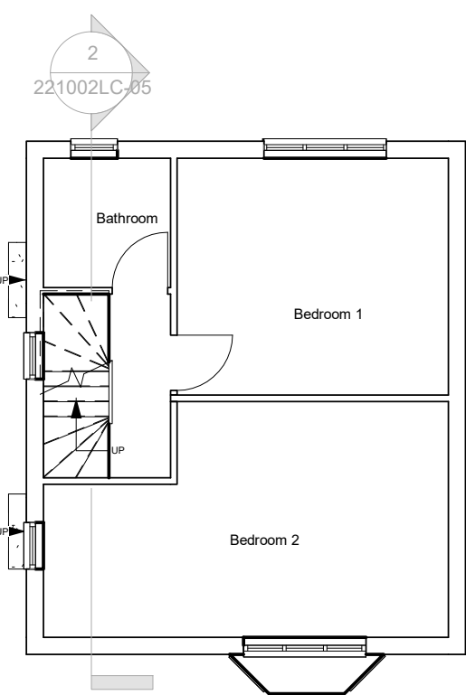
02. FF Proposed 1 : 100
