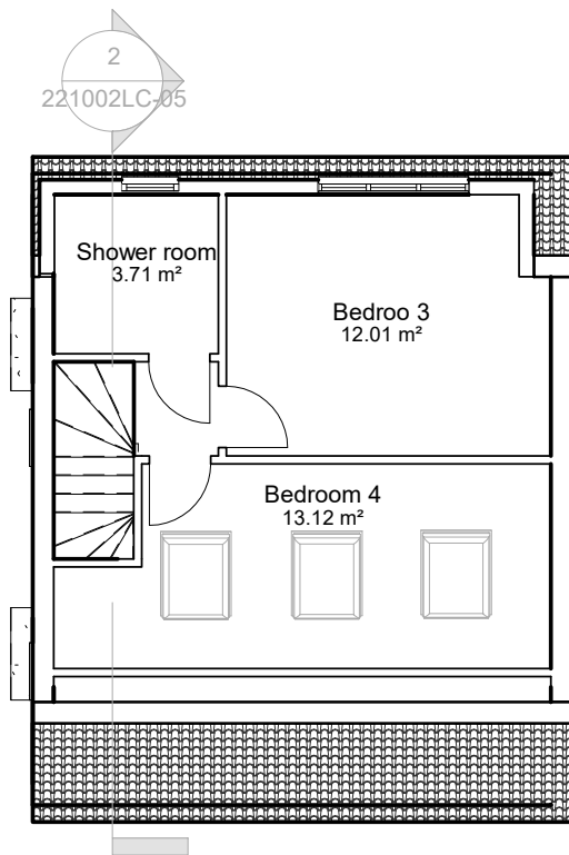
03. SF Proposed 1 : 100
