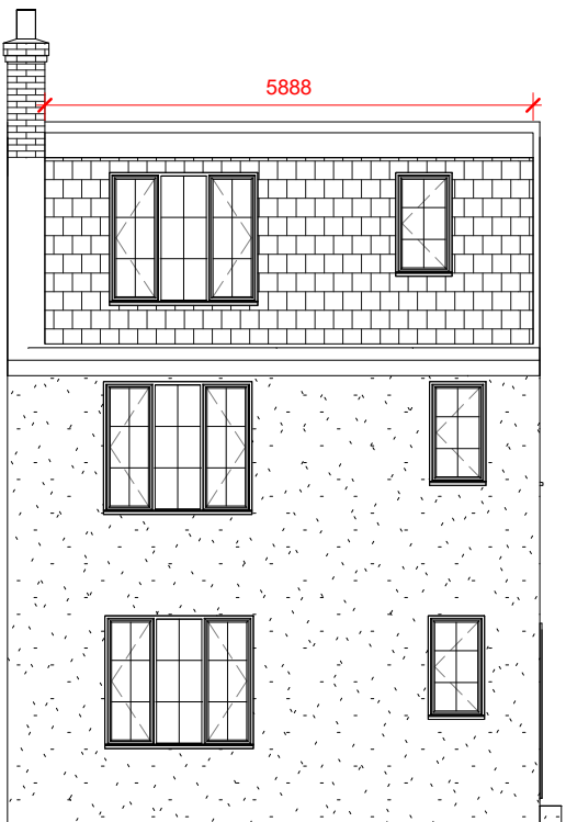
02. Rear Elevation Proposed 1 : 100
