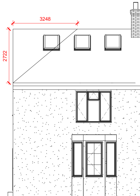
01. Front Elevation Proposed 1 : 100
