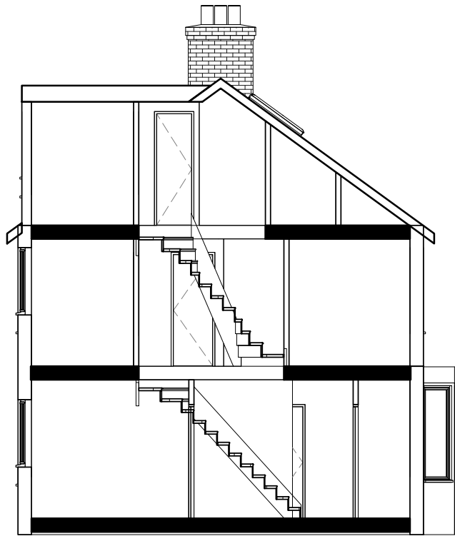
Section Proposed 1 : 100
