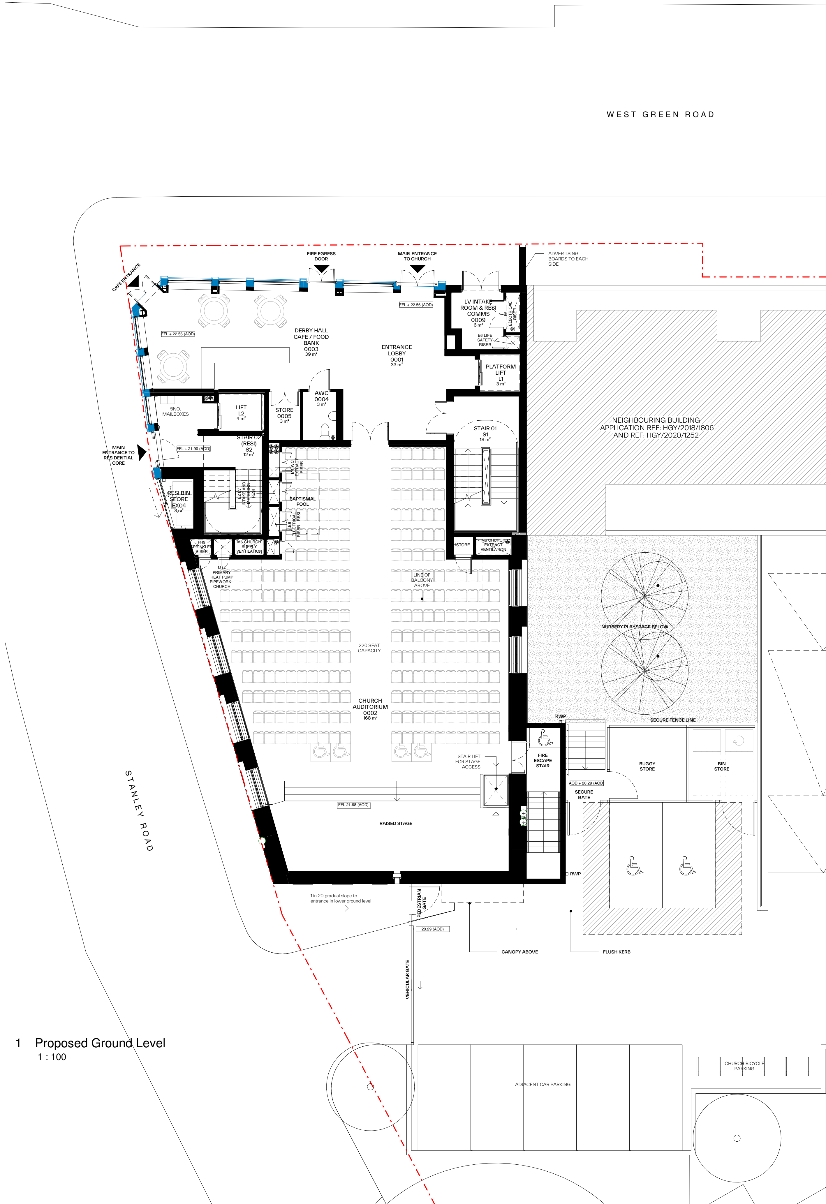
2 Proposed Level 01 1 : 100
