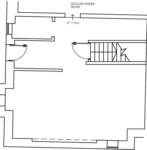
EXISTING BASEMENT FLOOR PLAN 1:100
