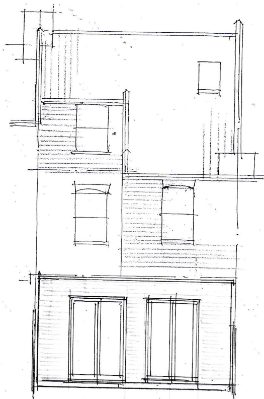
REAR ELEVATION
