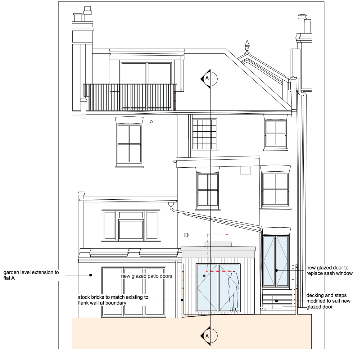
01 elevation_rear 1:100
