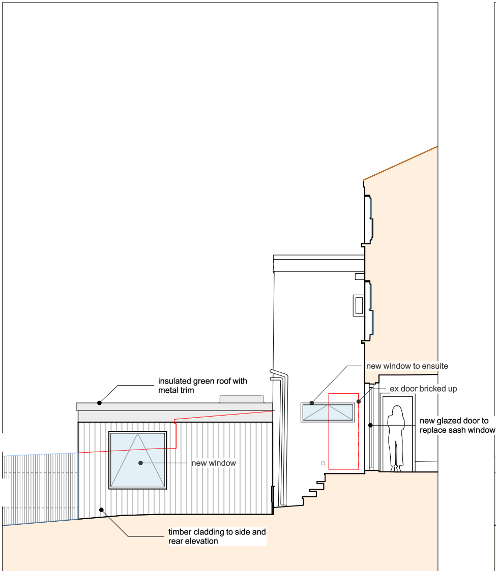
02 elevation_side 1:100
