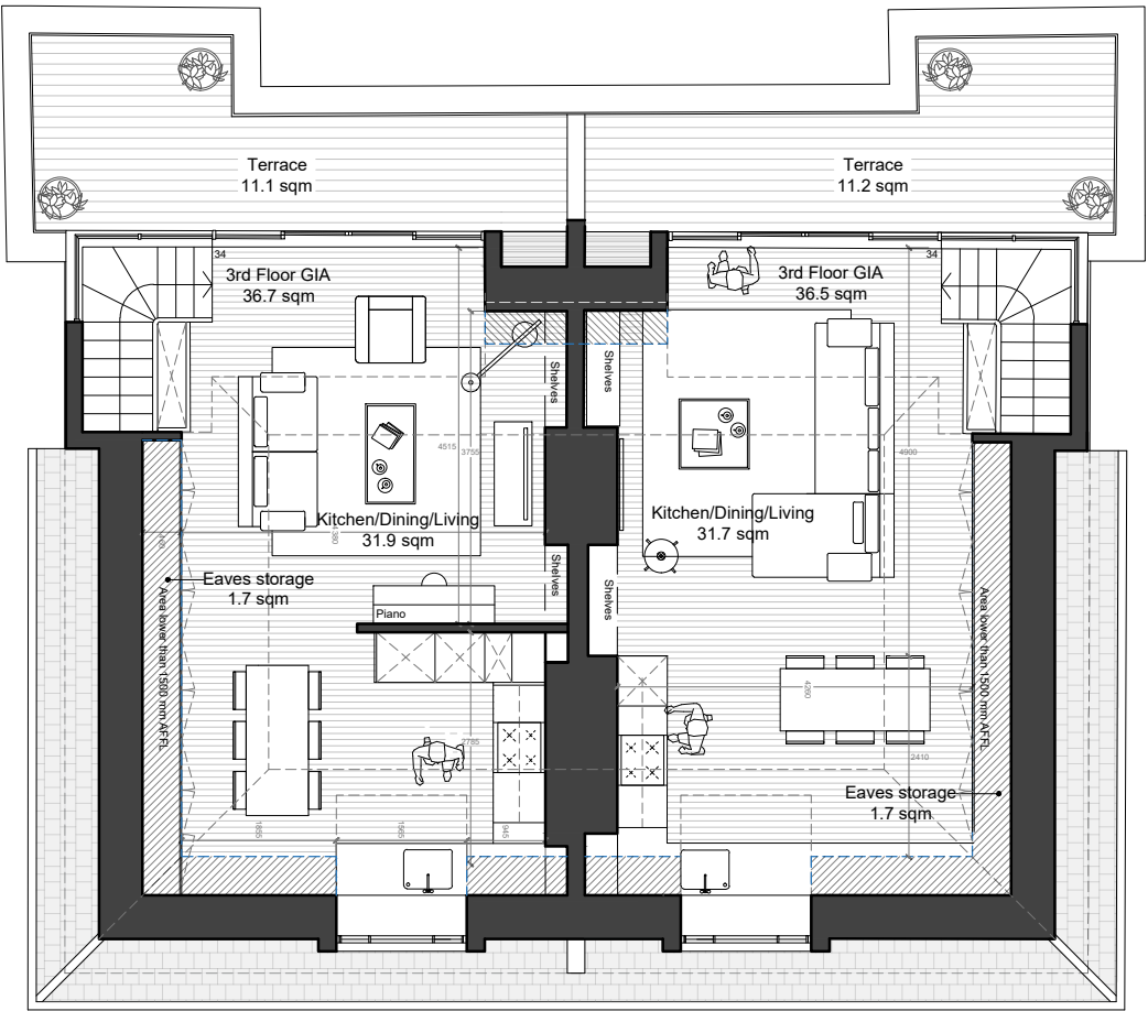
Proposed Third Floor Plan 1:100 @ A3
