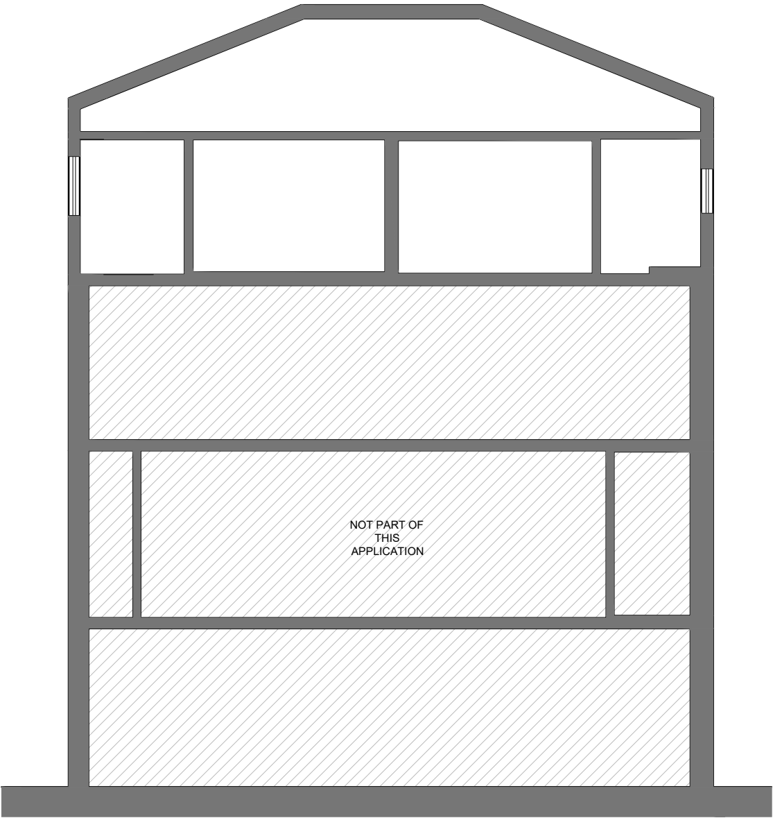
Existing Section AA 1:100 @ A3
