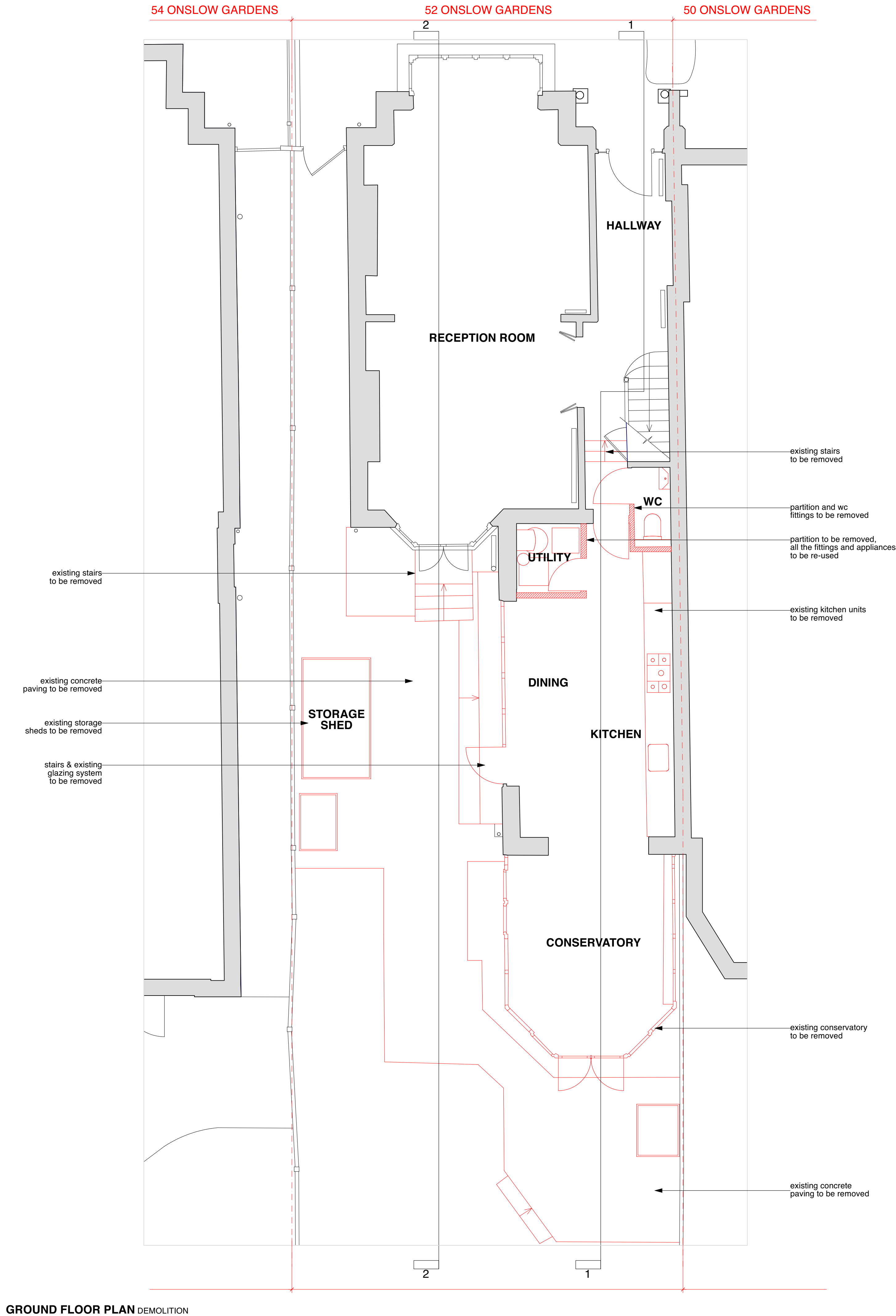
GROUND FLOOR PLAN DEMOLITION
