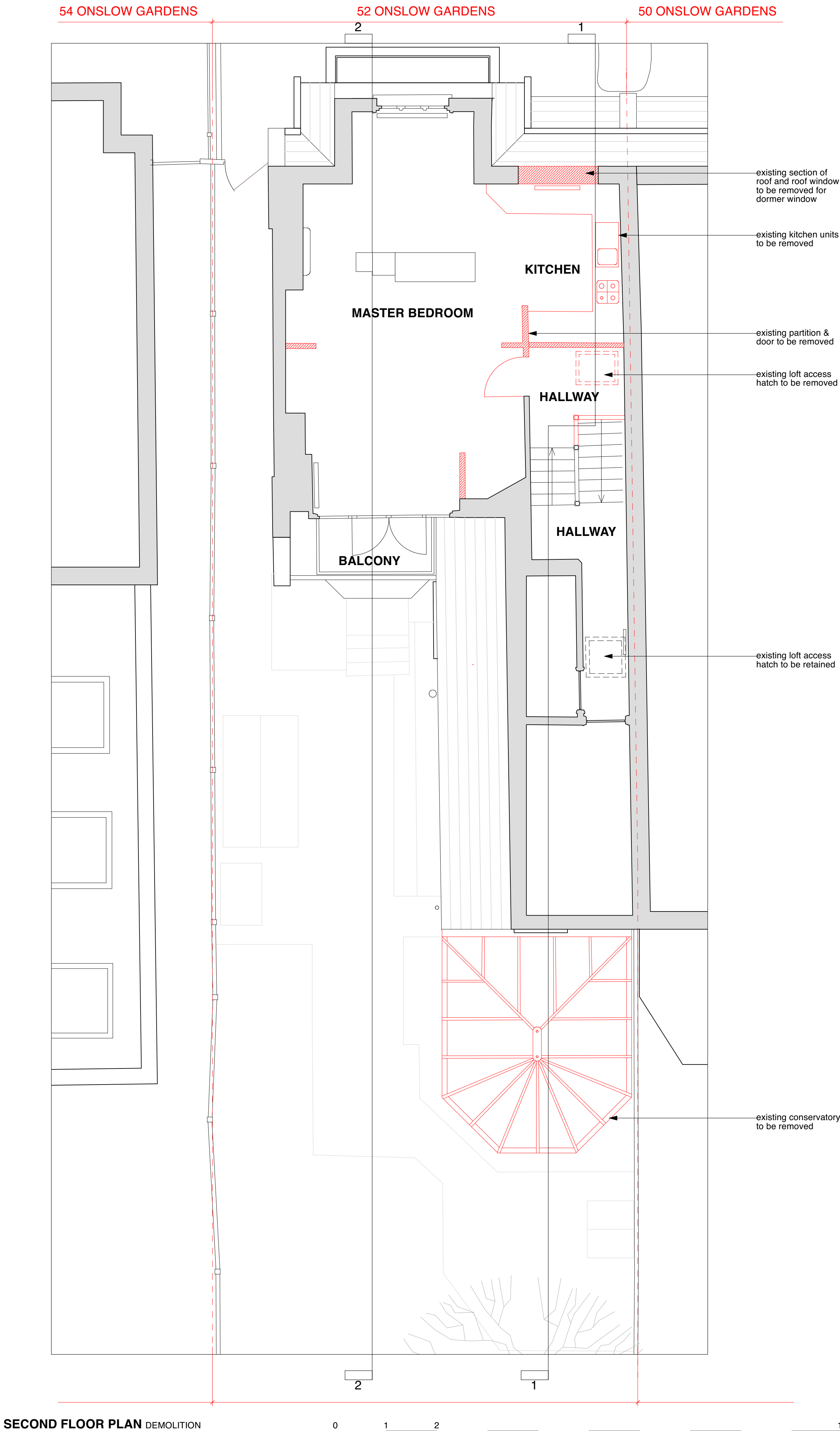
SECOND FLOOR PLAN DEMOLITION
