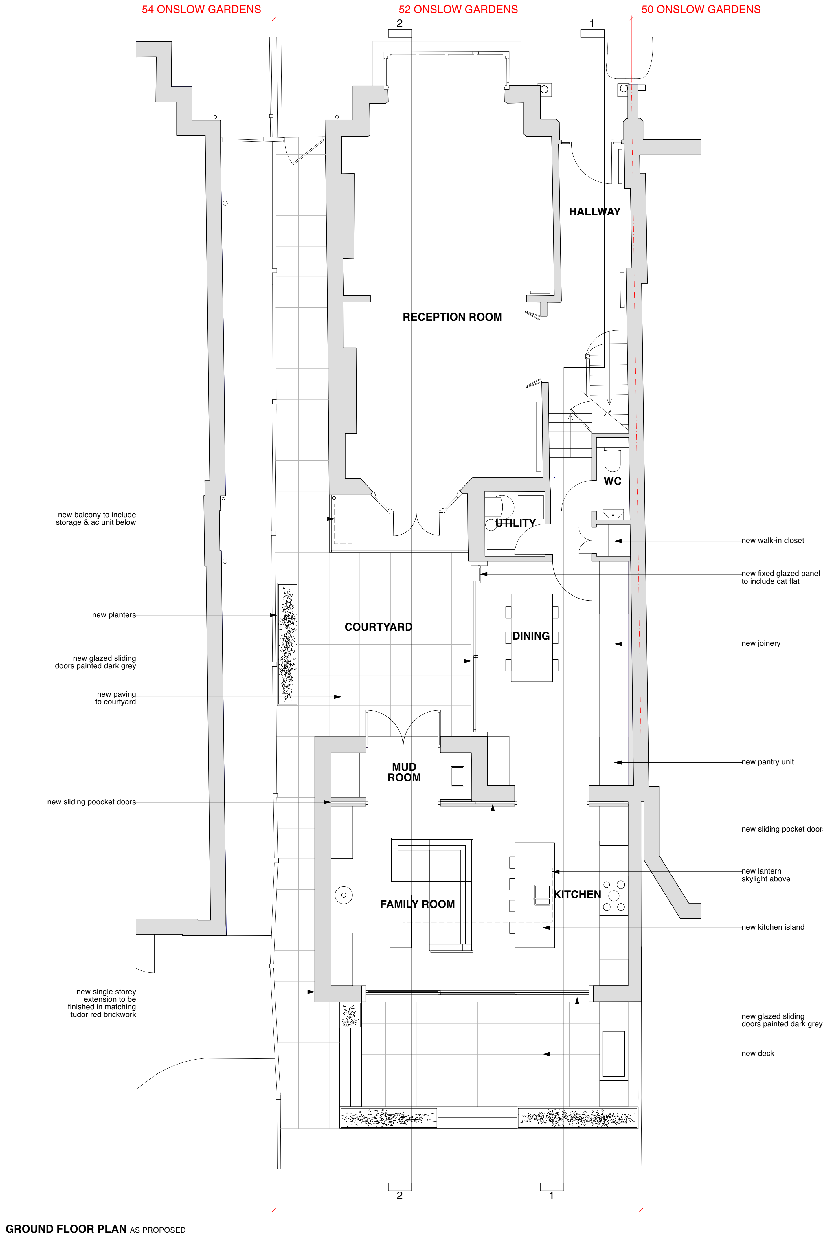
GROUND FLOOR PLAN AS PROPOSED
