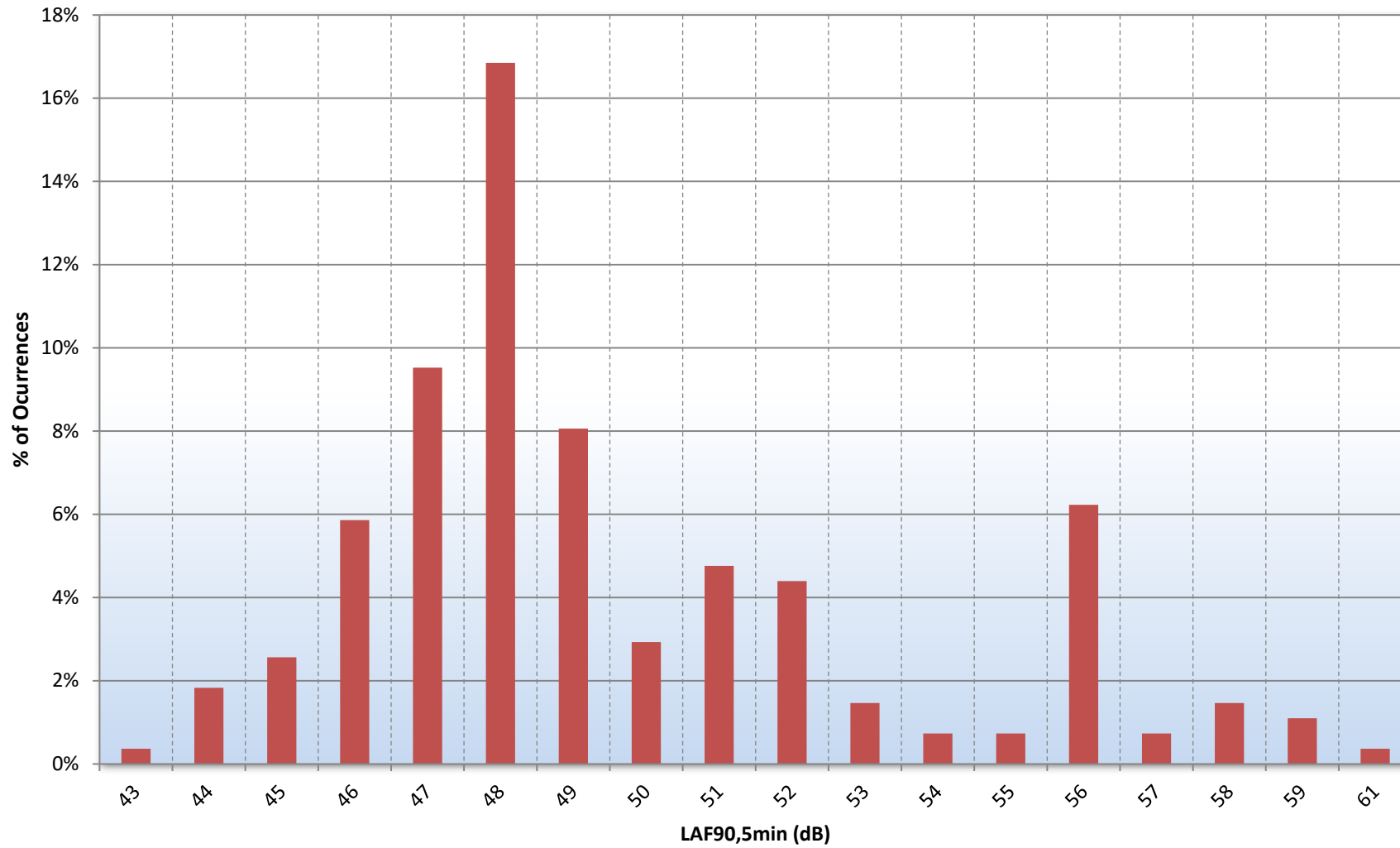
Figure 25564.Daytime L90.TH1
