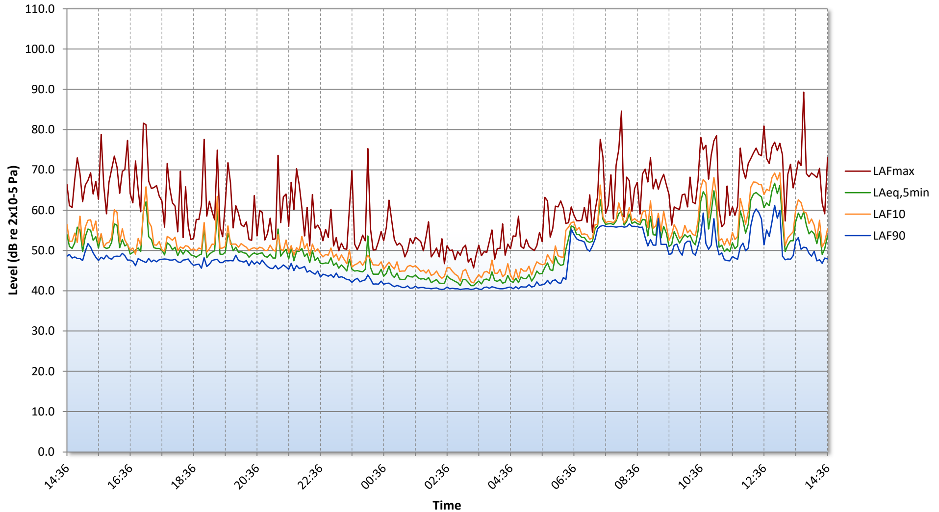
Figure 25564.TH1
