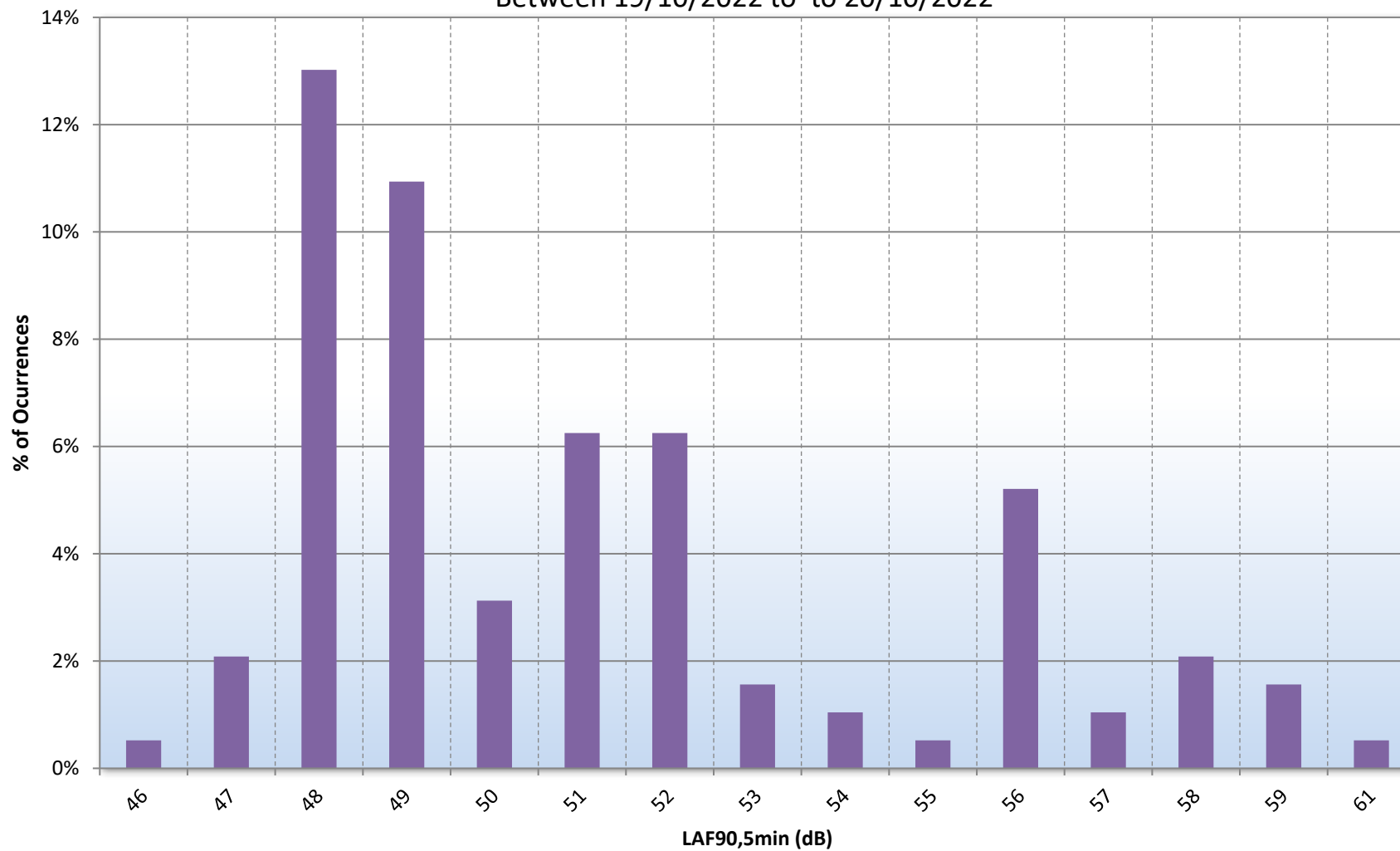
Figure 25564.Custom L90.TH1
