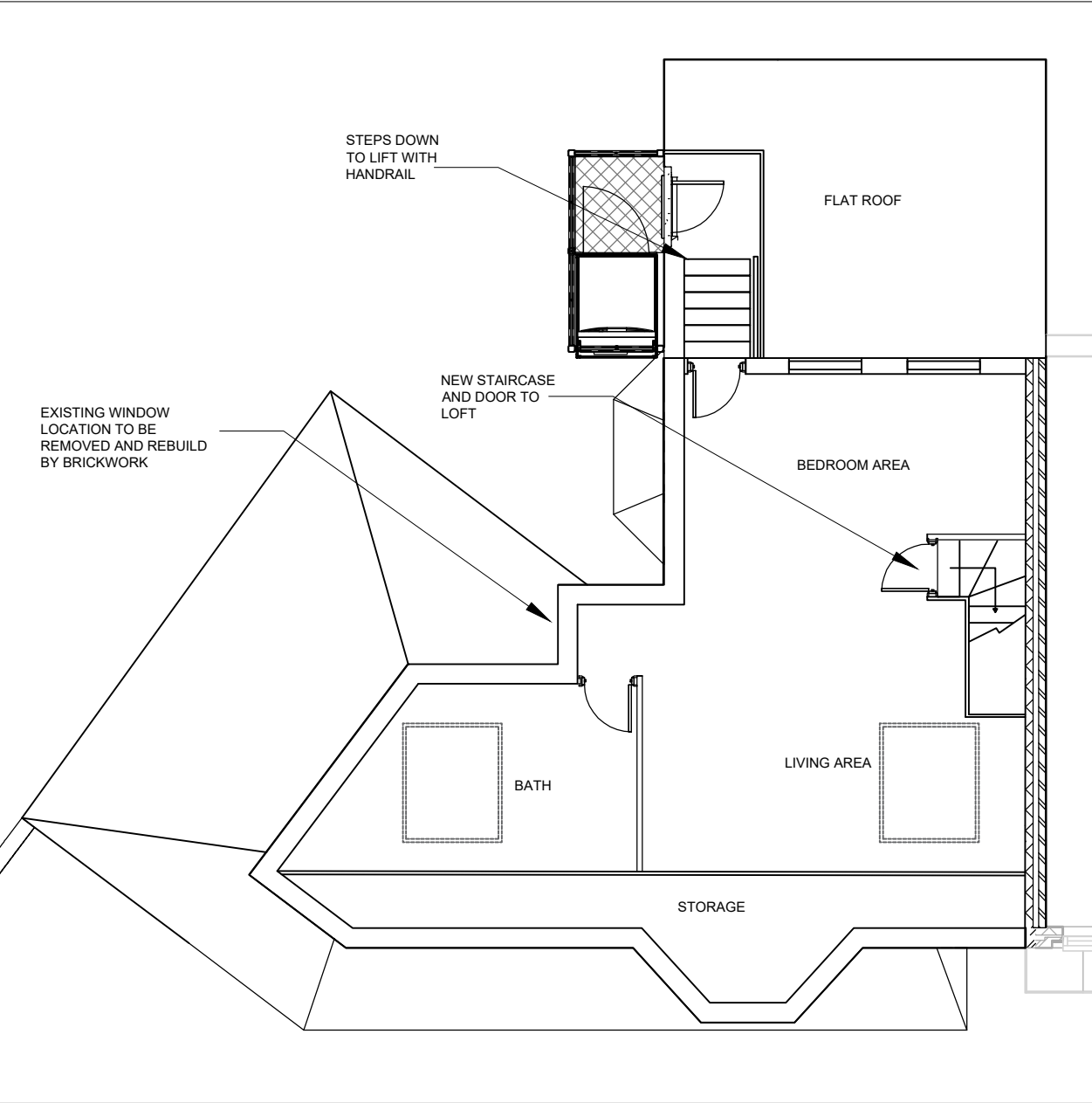
PROPOSED LOFT CONVERSION
