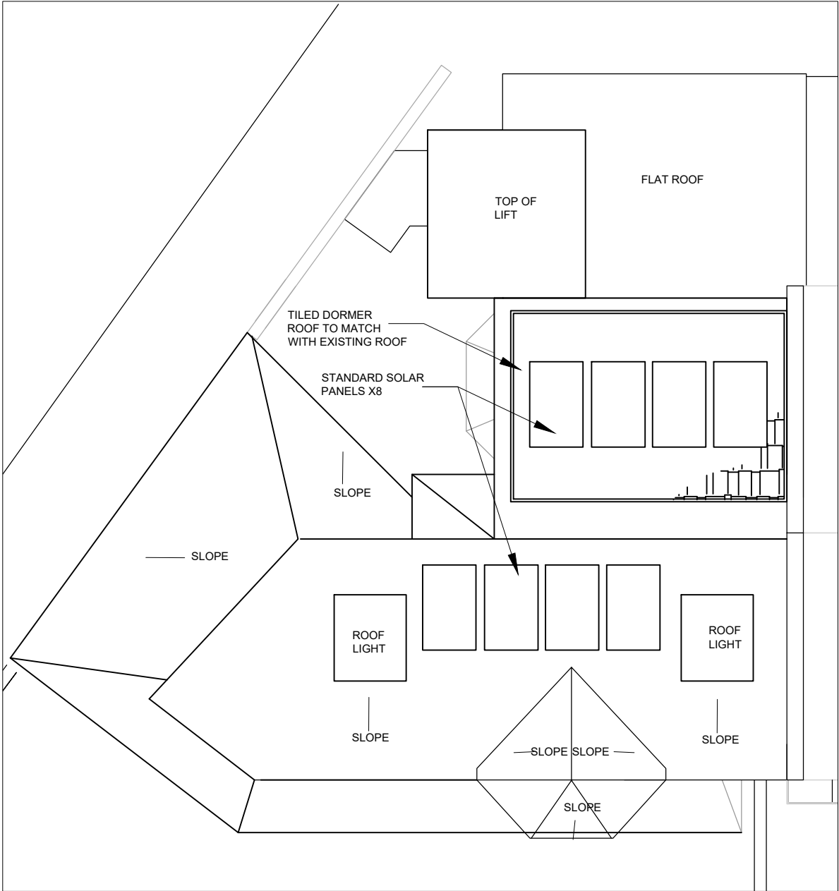
ROOF PLAN
