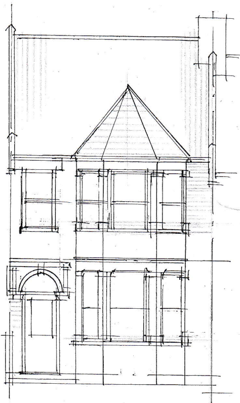
FRONT ELEVATION
